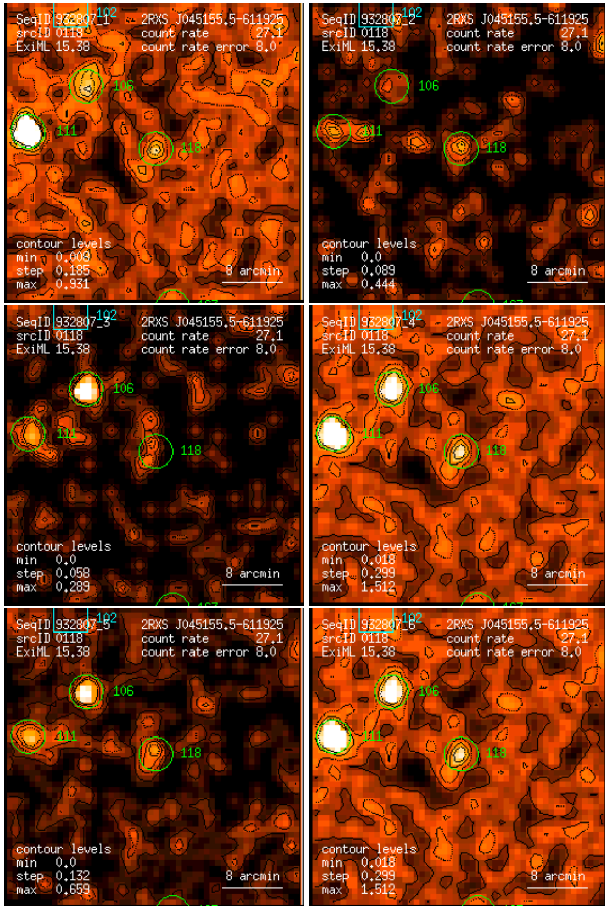
Figure 118: RASS 932807: detection 0118: band rate images, Gaussian filter: (1) PSPC channels 11 – 41, (2) 52 – 90, (3) 91 – 201, (4) 11 – 235, (5) 52 – 201, (6) 11 – 201. Broad band rates in counts/ks. Band rate contour levels in counts/ks/arcmin 2 .
