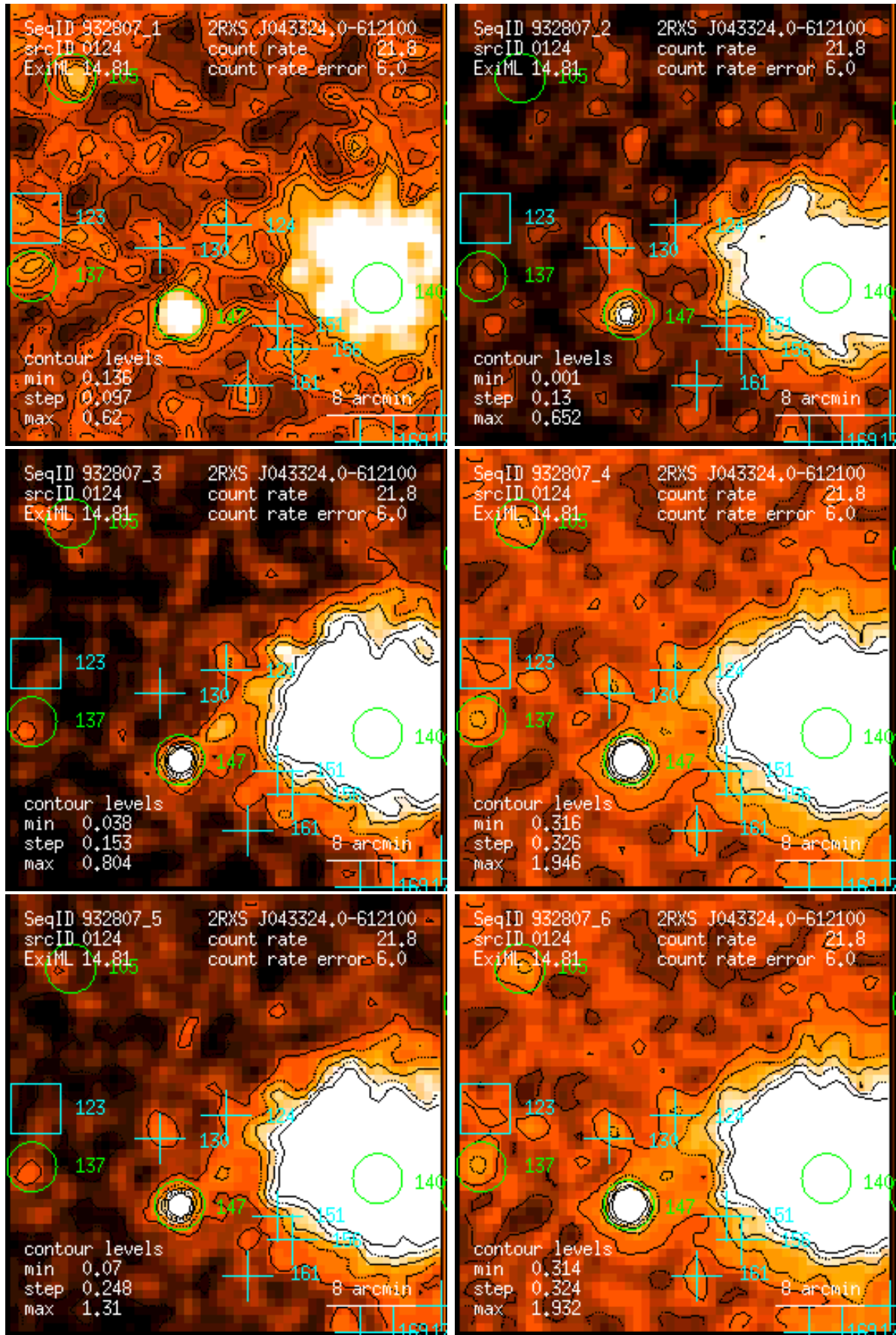
Figure 124: RASS 932807: detection 0124: band rate images, Gaussian filter: (1) PSPC channels 11 – 41, (2) 52 – 90, (3) 91 – 201, (4) 11 – 235, (5) 52 – 201, (6) 11 – 201. Broad band rates in counts/ks. Band rate contour levels in counts/ks/arcmin 2 .
