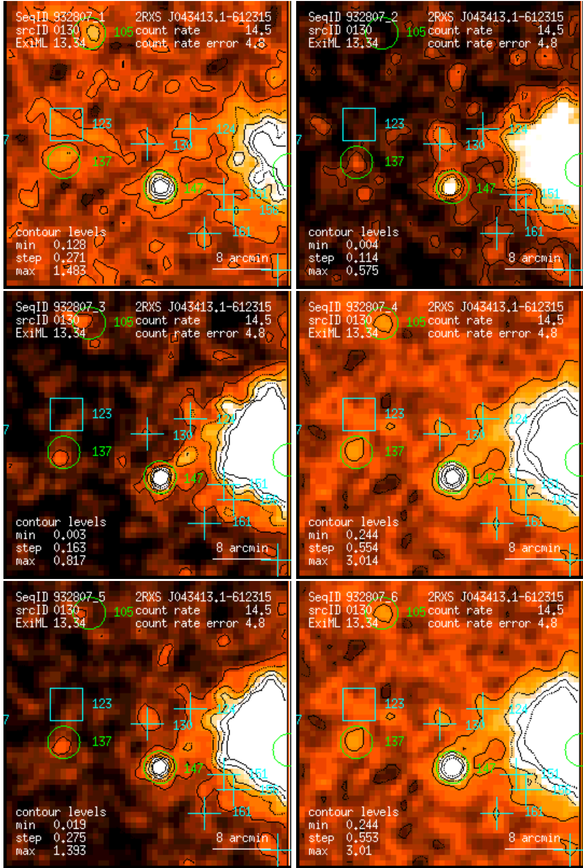
Figure 130: RASS 932807: detection 0130: band rate images, Gaussian filter: (1) PSPC channels 11 – 41, (2) 52 – 90, (3) 91 – 201, (4) 11 – 235, (5) 52 – 201, (6) 11 – 201. Broad band rates in counts/ks. Band rate contour levels in counts/ks/arcmin 2 .
