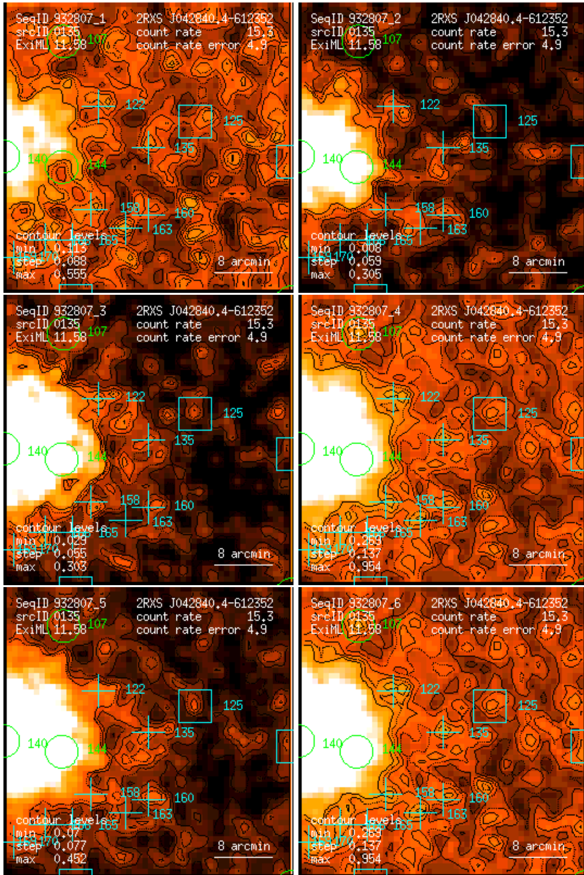
Figure 135: RASS 932807: detection 0135: band rate images, Gaussian filter: (1) PSPC channels 11 – 41, (2) 52 – 90, (3) 91 – 201, (4) 11 – 235, (5) 52 – 201, (6) 11 – 201. Broad band rates in counts/ks. Band rate contour levels in counts/ks/arcmin 2 .
