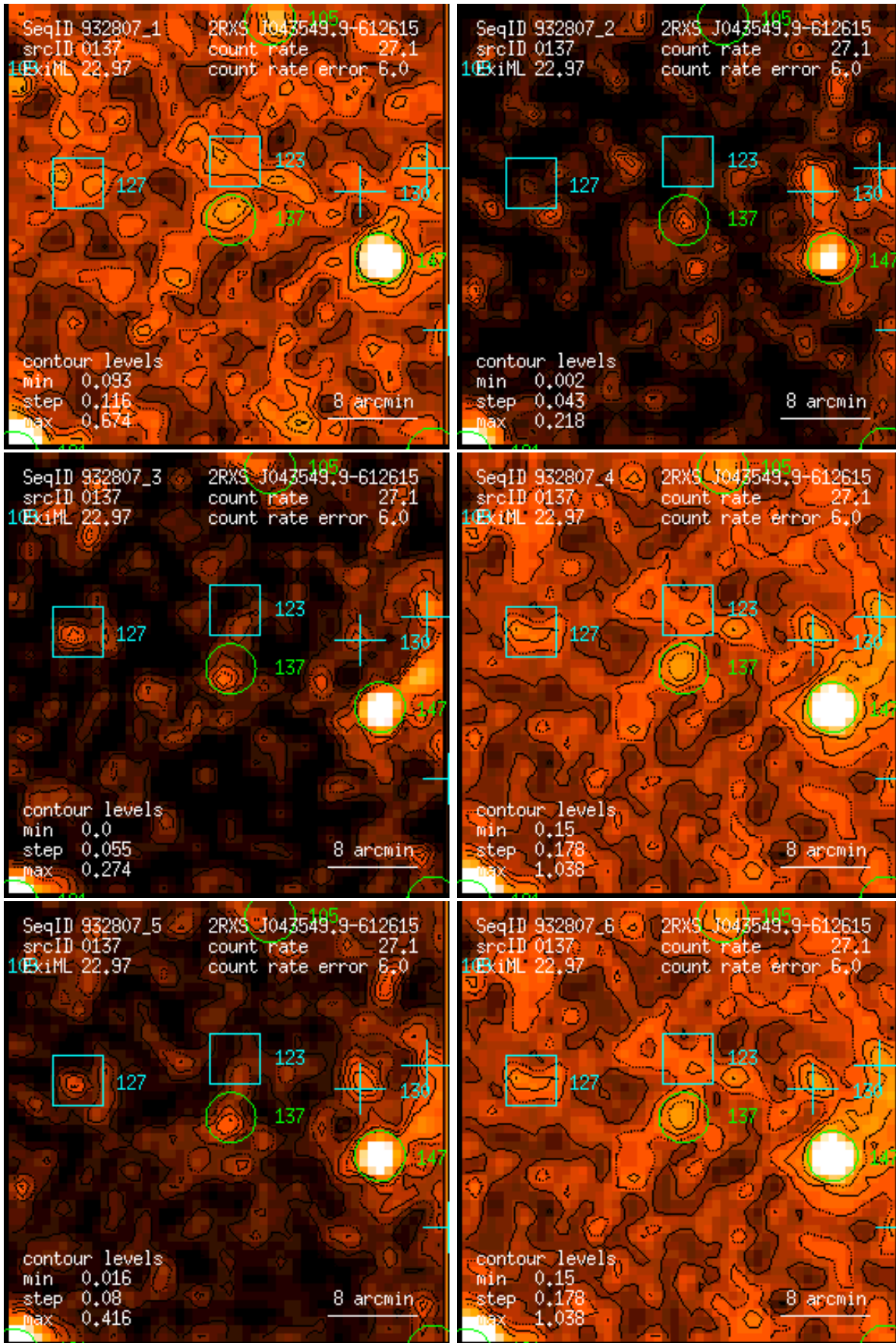
Figure 137: RASS 932807: detection 0137: band rate images, Gaussian filter: (1) PSPC channels 11 – 41, (2) 52 – 90, (3) 91 – 201, (4) 11 – 235, (5) 52 – 201, (6) 11 – 201. Broad band rates in counts/ks. Band rate contour levels in counts/ks/arcmin 2 .
