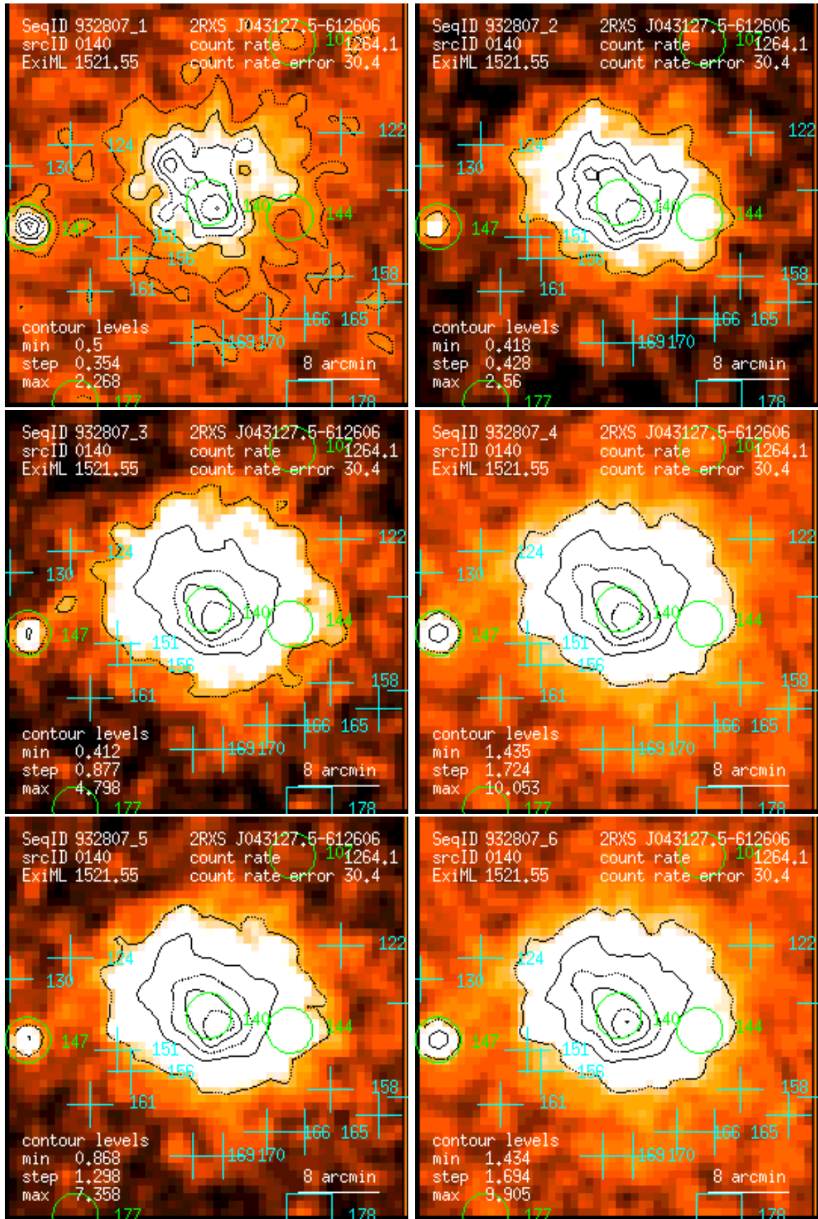
Figure 140: RASS 932807: detection 0140: band rate images, Gaussian filter: (1) PSPC channels 11 – 41, (2) 52 – 90, (3) 91 – 201, (4) 11 – 235, (5) 52 – 201, (6) 11 – 201. Broad band rates in counts/ks. Band rate contour levels in counts/ks/arcmin 2 .
