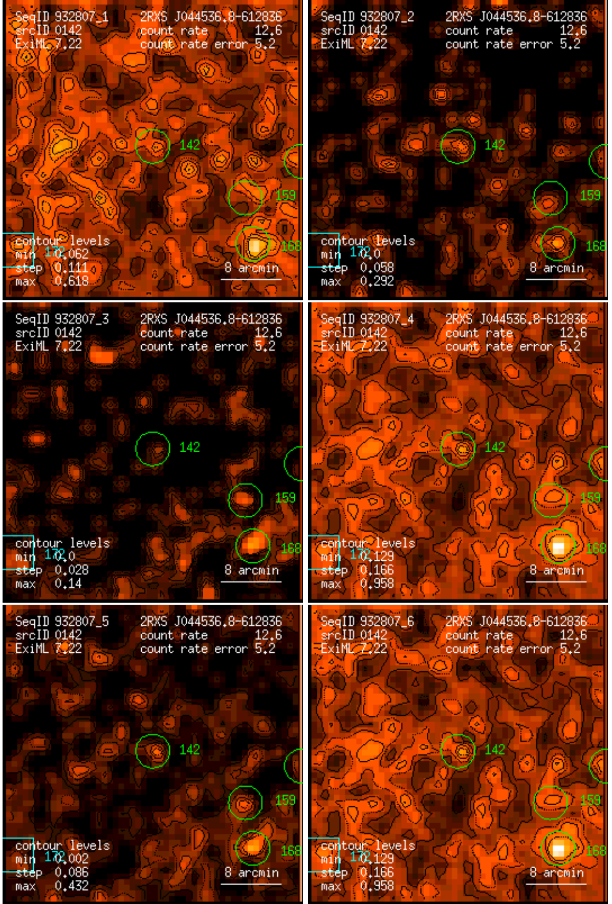
Figure 142: RASS 932807: detection 0142: band rate images, Gaussian filter: (1) PSPC channels 11 – 41, (2) 52 – 90, (3) 91 – 201, (4) 11 – 235, (5) 52 – 201, (6) 11 – 201. Broad band rates in counts/ks. Band rate contour levels in counts/ks/arcmin 2 .
