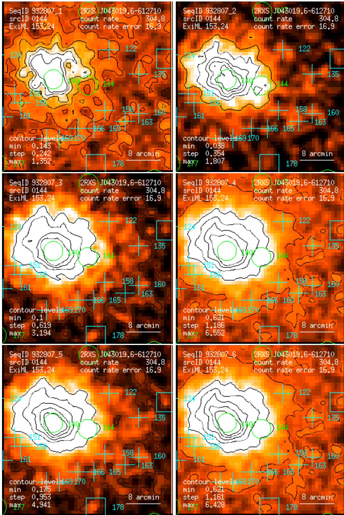
Figure 144: RASS 932807: detection 0144: band rate images, Gaussian filter: (1) PSPC channels 11 – 41, (2) 52 – 90, (3) 91 – 201, (4) 11 – 235, (5) 52 – 201, (6) 11 – 201. Broad band rates in counts/ks. Band rate contour levels in counts/ks/arcmin 2 .
