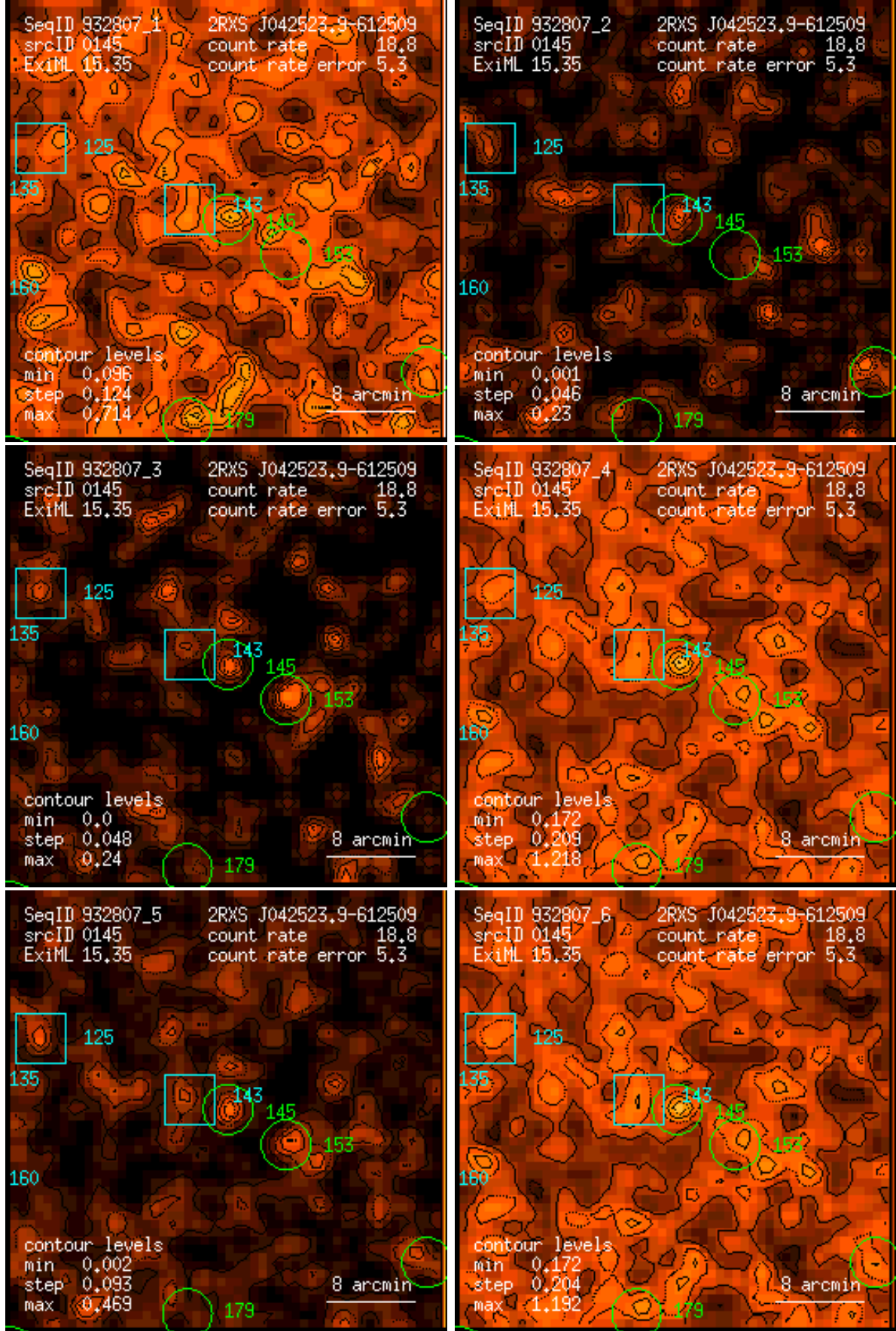
Figure 145: RASS 932807: detection 0145: band rate images, Gaussian filter: (1) PSPC channels 11 – 41, (2) 52 – 90, (3) 91 – 201, (4) 11 – 235, (5) 52 – 201, (6) 11 – 201. Broad band rates in counts/ks. Band rate contour levels in counts/ks/arcmin 2 .
