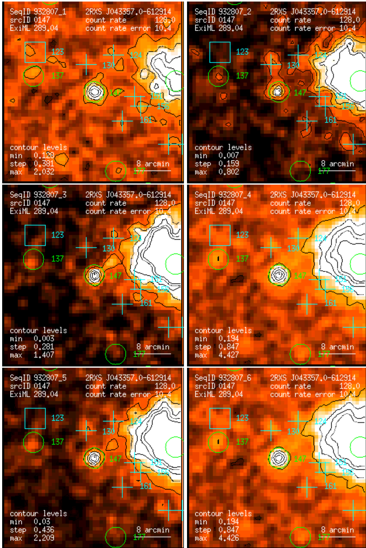
Figure 147: RASS 932807: detection 0147: band rate images, Gaussian filter: (1) PSPC channels 11 – 41, (2) 52 – 90, (3) 91 – 201, (4) 11 – 235, (5) 52 – 201, (6) 11 – 201. Broad band rates in counts/ks. Band rate contour levels in counts/ks/arcmin 2 .
