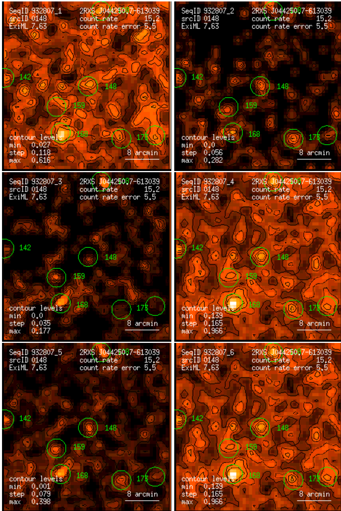
Figure 148: RASS 932807: detection 0148: band rate images, Gaussian filter: (1) PSPC channels 11 – 41, (2) 52 – 90, (3) 91 – 201, (4) 11 – 235, (5) 52 – 201, (6) 11 – 201. Broad band rates in counts/ks. Band rate contour levels in counts/ks/arcmin 2 .
