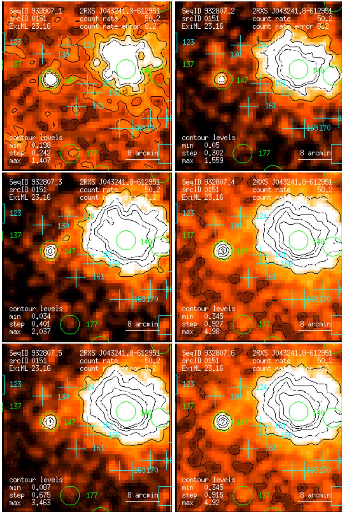
Figure 151: RASS 932807: detection 0151: band rate images, Gaussian filter: (1) PSPC channels 11 – 41, (2) 52 – 90, (3) 91 – 201, (4) 11 – 235, (5) 52 – 201, (6) 11 – 201. Broad band rates in counts/ks. Band rate contour levels in counts/ks/arcmin 2 .
