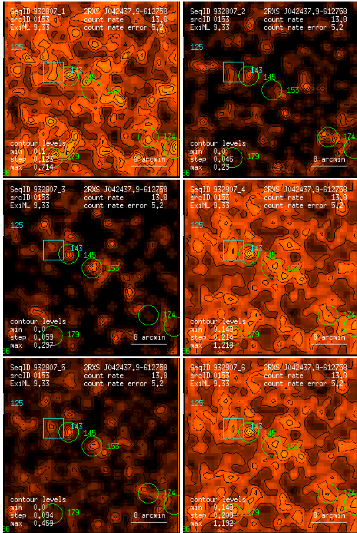
Figure 153: RASS 932807: detection 0153: band rate images, Gaussian filter: (1) PSPC channels 11 – 41, (2) 52 – 90, (3) 91 – 201, (4) 11 – 235, (5) 52 – 201, (6) 11 – 201. Broad band rates in counts/ks. Band rate contour levels in counts/ks/arcmin 2 .
