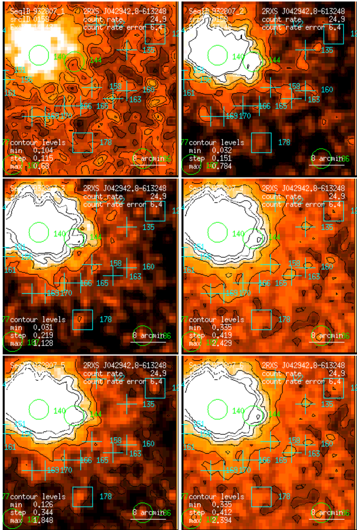
Figure 158: RASS 932807: detection 0158: band rate images, Gaussian filter: (1) PSPC channels 11 – 41, (2) 52 – 90, (3) 91 – 201, (4) 11 – 235, (5) 52 – 201, (6) 11 – 201. Broad band rates in counts/ks. Band rate contour levels in counts/ks/arcmin 2 .
