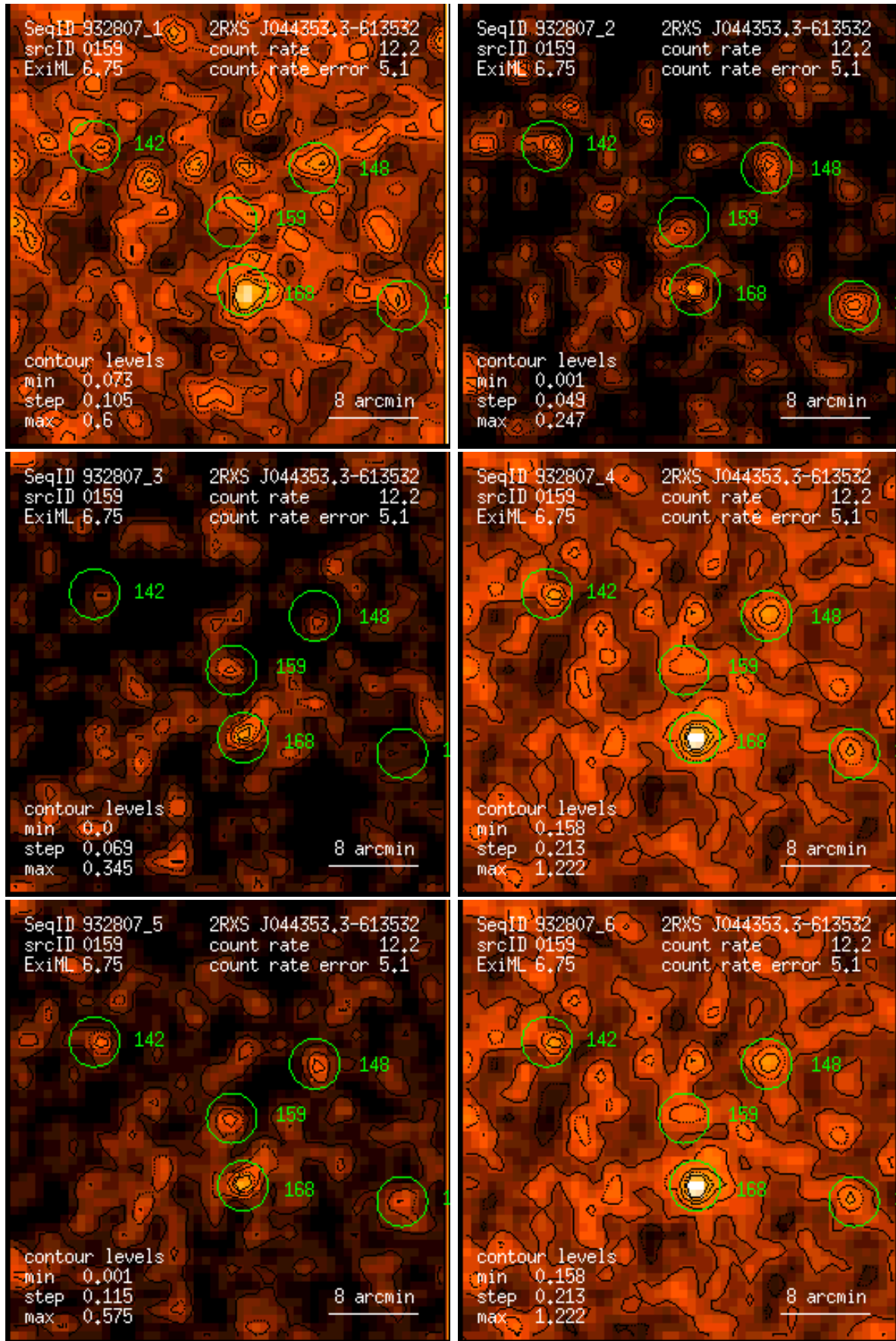
Figure 159: RASS 932807: detection 0159: band rate images, Gaussian filter: (1) PSPC channels 11 – 41, (2) 52 – 90, (3) 91 – 201, (4) 11 – 235, (5) 52 – 201, (6) 11 – 201. Broad band rates in counts/ks. Band rate contour levels in counts/ks/arcmin 2 .
