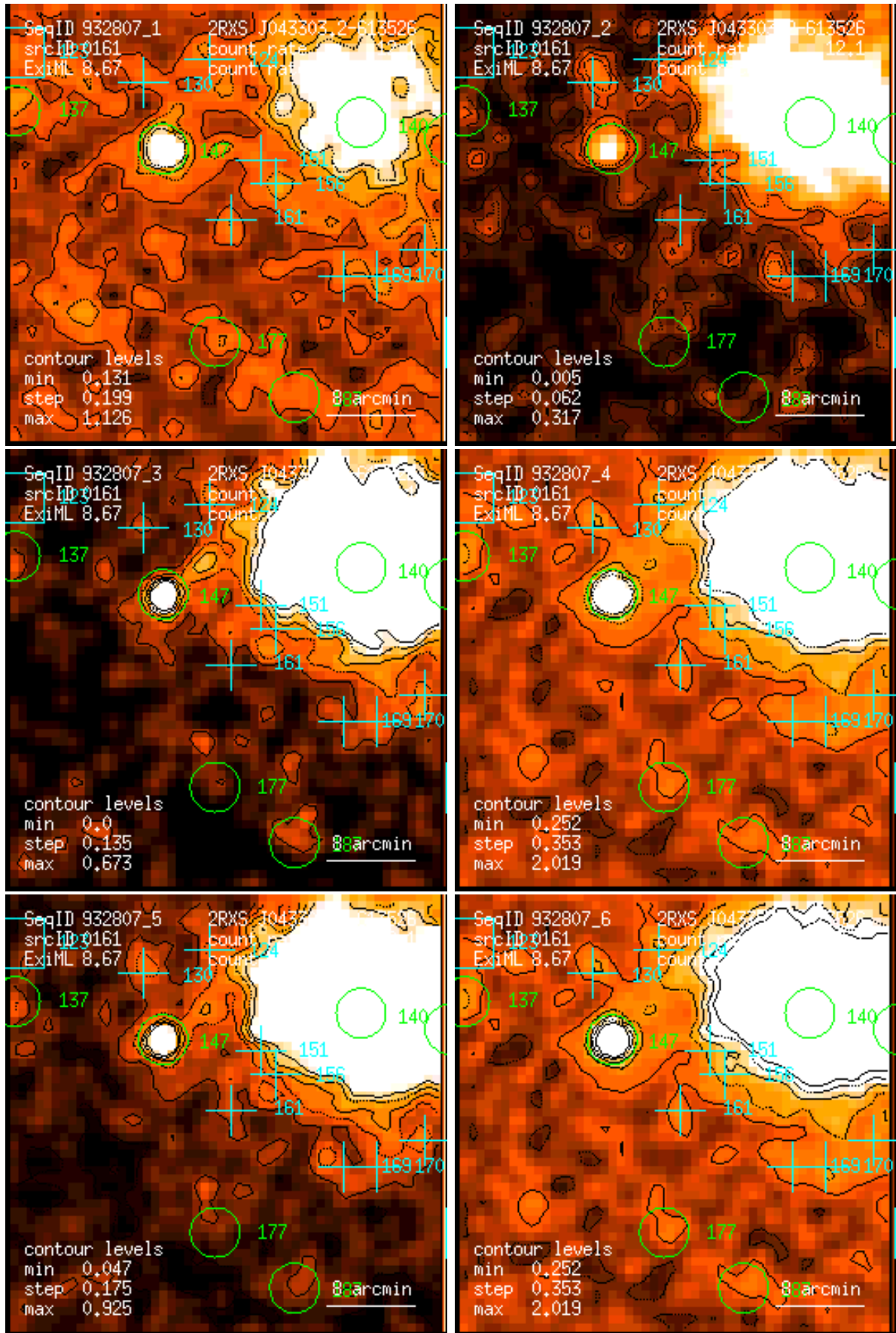
Figure 161: RASS 932807: detection 0161: band rate images, Gaussian filter: (1) PSPC channels 11 – 41, (2) 52 – 90, (3) 91 – 201, (4) 11 – 235, (5) 52 – 201, (6) 11 – 201. Broad band rates in counts/ks. Band rate contour levels in counts/ks/arcmin 2 .
