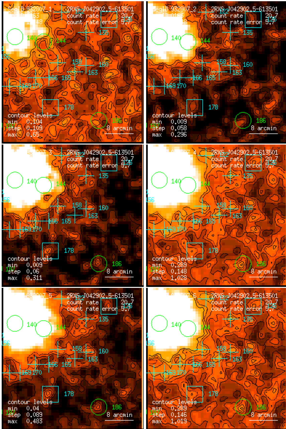
Figure 163: RASS 932807: detection 0163: band rate images, Gaussian filter: (1) PSPC channels 11 – 41, (2) 52 – 90, (3) 91 – 201, (4) 11 – 235, (5) 52 – 201, (6) 11 – 201. Broad band rates in counts/ks. Band rate contour levels in counts/ks/arcmin 2 .
