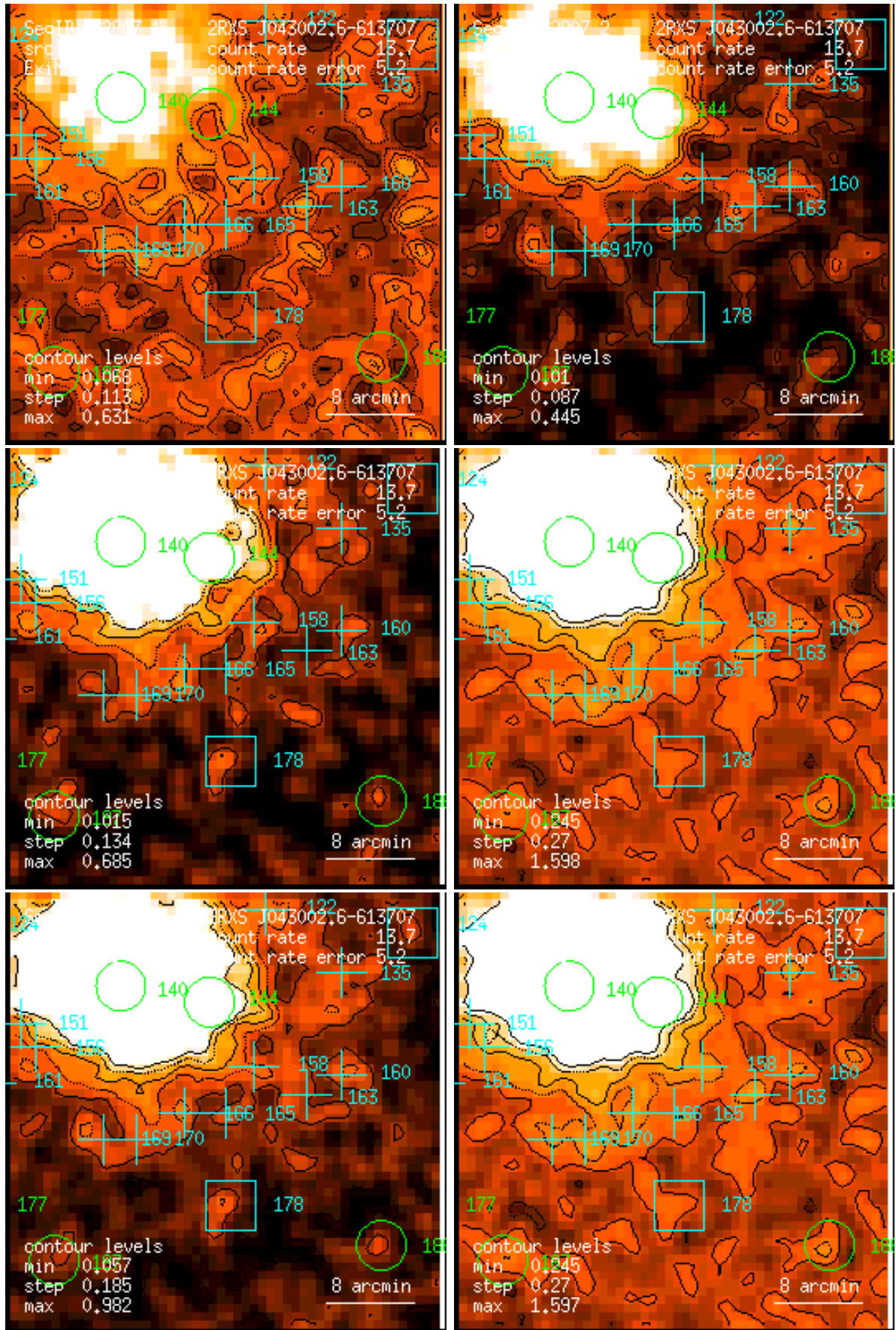
Figure 165: RASS 932807: detection 0165: band rate images, Gaussian filter: (1) PSPC channels 11 – 41, (2) 52 – 90, (3) 91 – 201, (4) 11 – 235, (5) 52 – 201, (6) 11 – 201. Broad band rates in counts/ks. Band rate contour levels in counts/ks/arcmin 2 .
