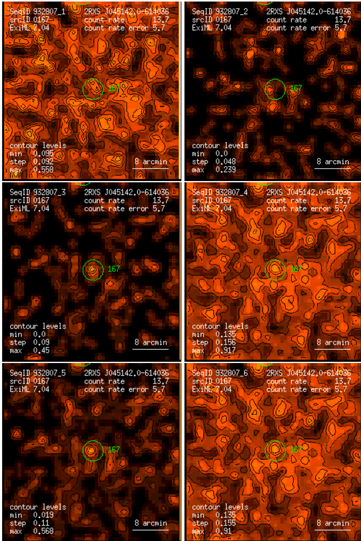
Figure 167: RASS 932807: detection 0167: band rate images, Gaussian filter: (1) PSPPC channels 11 – 41, (2) 52 – 90, (3) 91 – 201, (4) 11 – 235, (5) 52 – 201, (6) 11 – 201. Broad band rates in counts/ks. Band rate contour levels in counts/ks/arcmin 2 .
