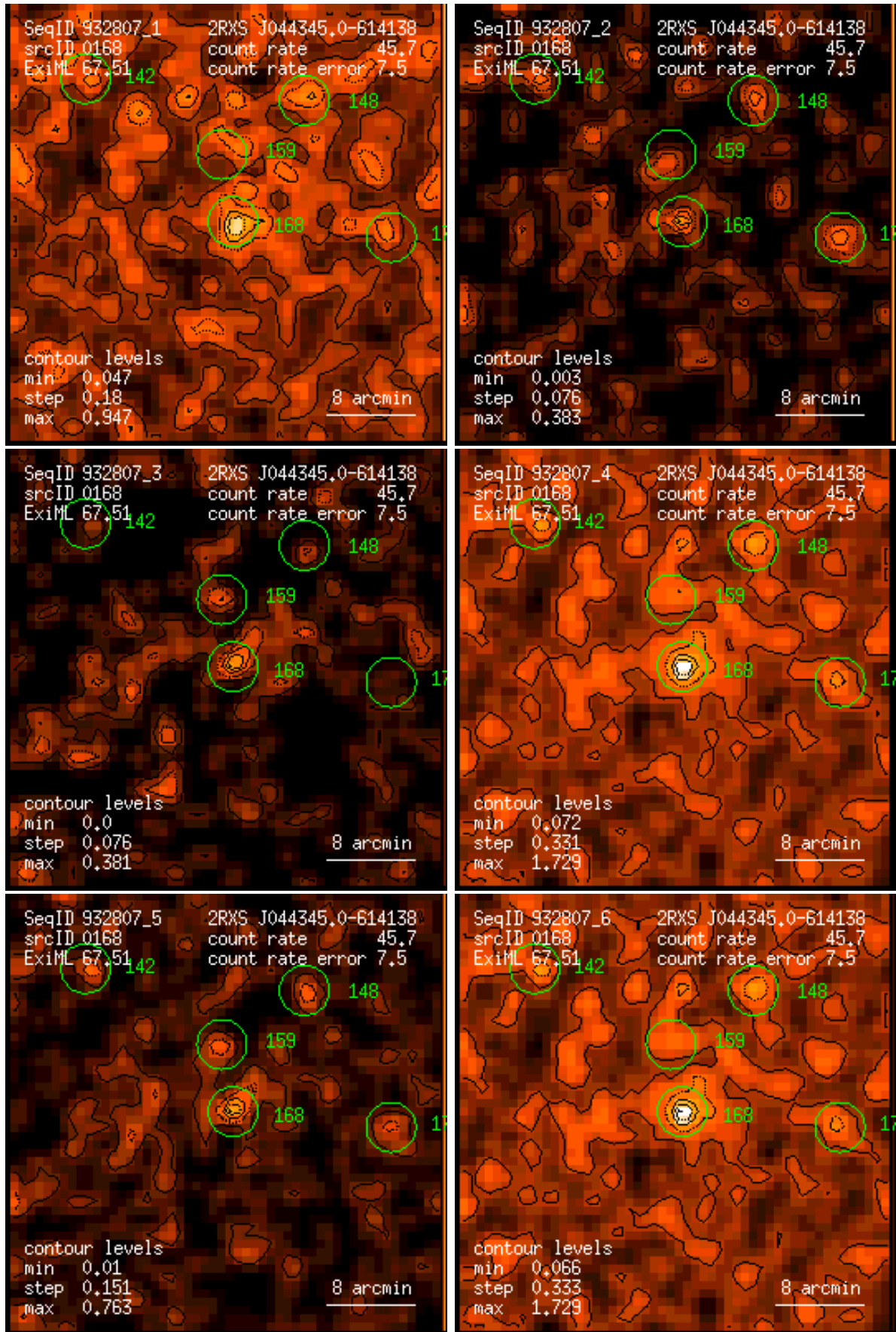
Figure 168: RASS 932807: detection 0168: band rate images, Gaussian filter: (1) PSPC channels 11 – 41, (2) 52 – 90, (3) 91 – 201, (4) 11 – 235, (5) 52 – 201, (6) 11 – 201. Broad band rates in counts/ks. Band rate contour levels in counts/ks/arcmin 2 .
