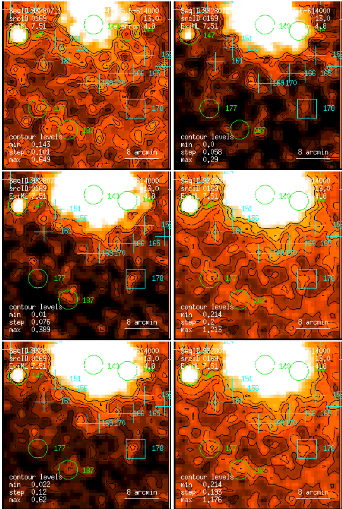
Figure 169: RASS 932807: detection 0169: band rate images, Gaussian filter: (1) PSPC channels 11 – 41, (2) 52 – 90, (3) 91 – 201, (4) 11 – 235, (5) 52 – 201, (6) 11 – 201. Broad band rates in counts/ks. Band rate contour levels in counts/ks/arcmin 2 .
