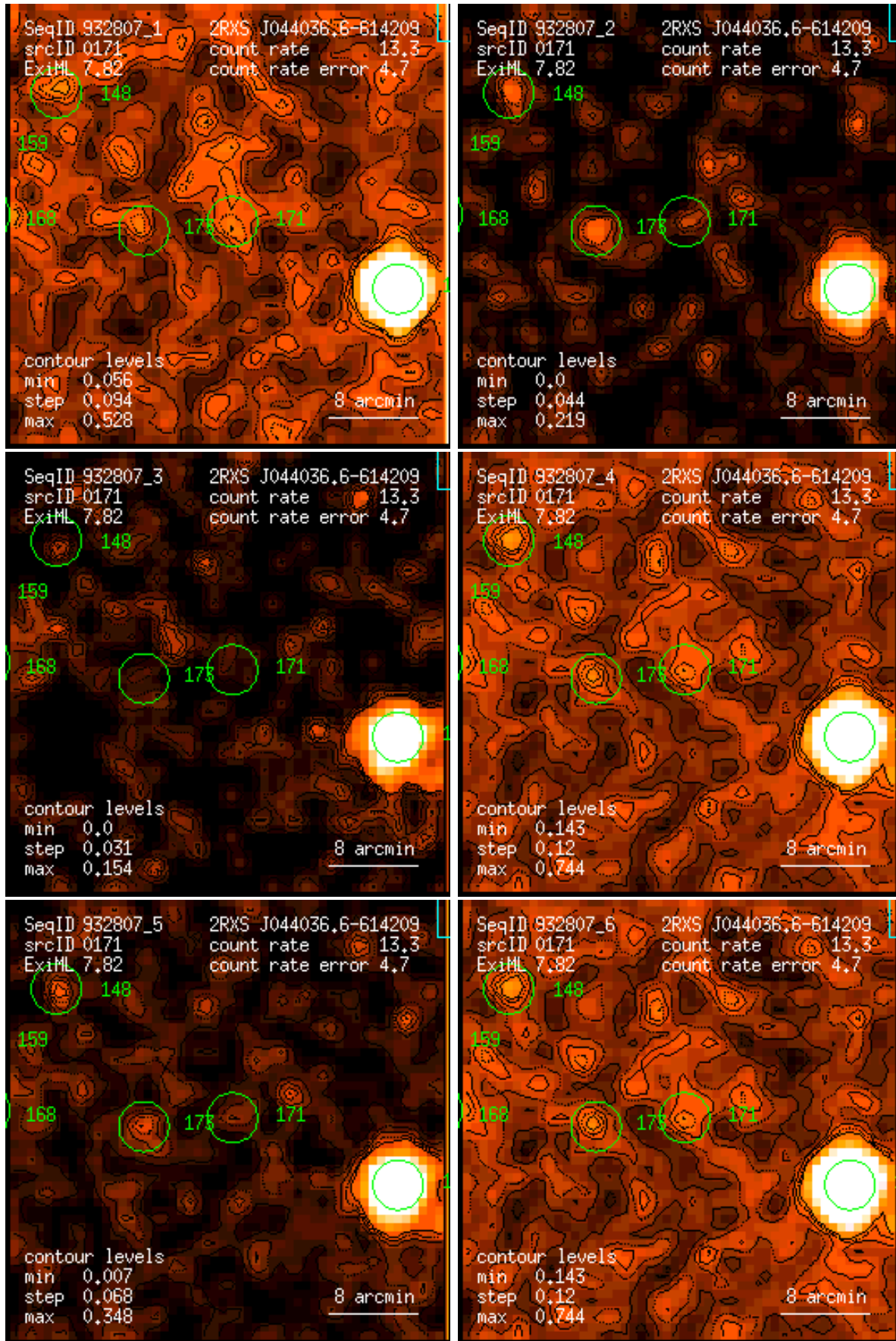
Figure 171: RASS 932807: detection 0171: band rate images, Gaussian filter: (1) PSPC channels 11 – 41, (2) 52 – 90, (3) 91 – 201, (4) 11 – 235, (5) 52 – 201, (6) 11 – 201. Broad band rates in counts/ks. Band rate contour levels in counts/ks/arcmin 2 .
