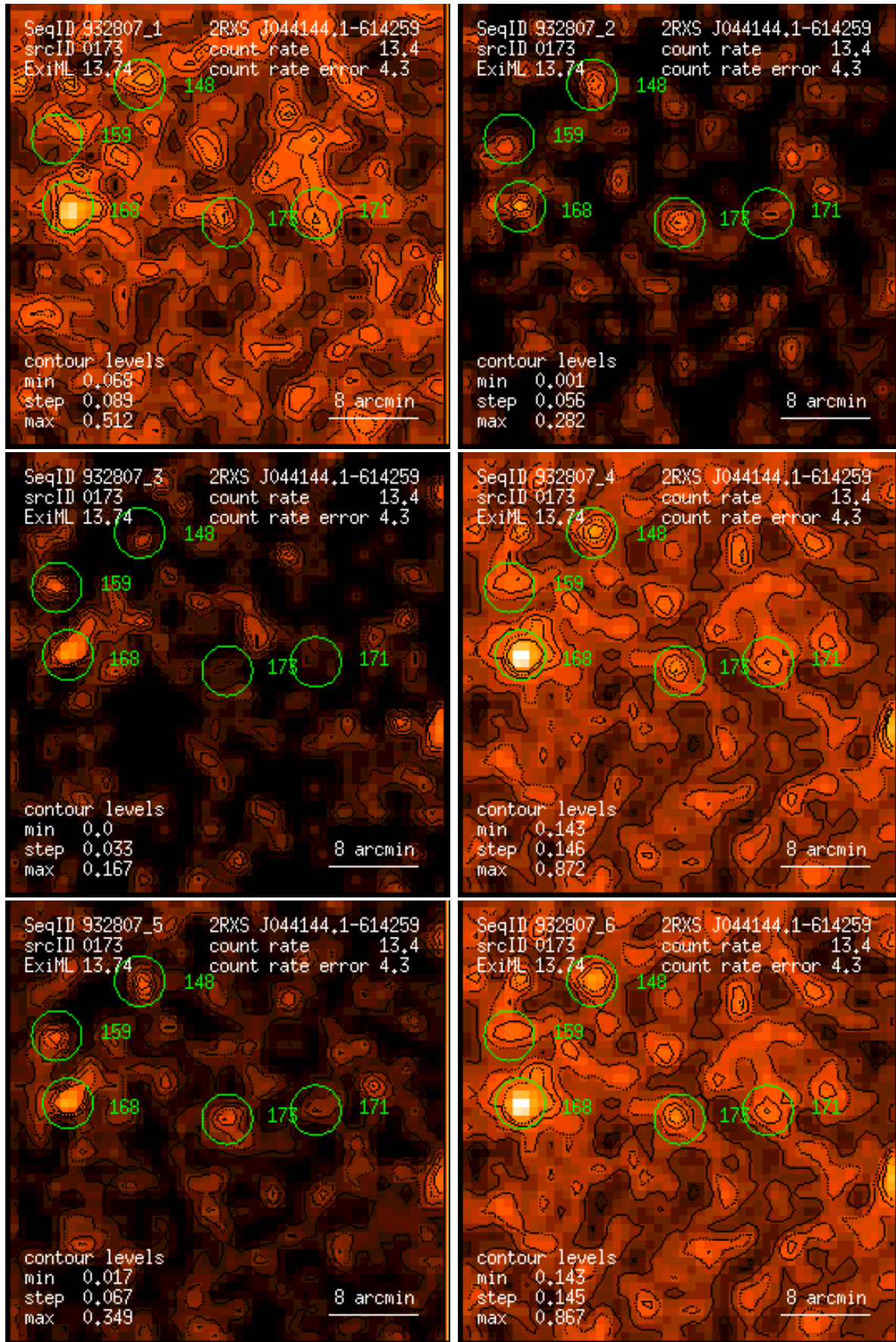
Figure 173: RASS 932807: detection 0173: band rate images, Gaussian filter: (1) PSPC channels 11 – 41, (2) 52 – 90, (3) 91 – 201, (4) 11 – 235, (5) 52 – 201, (6) 11 – 201. Broad band rates in counts/ks. Band rate contour levels in counts/ks/arcmin 2 .
