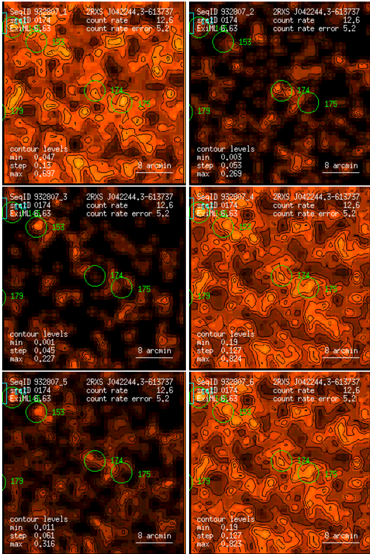
Figure 174: RASS 932807: detection 0174: band rate images, Gaussian filter: (1) PSPC channels 11 – 41, (2) 52 – 90, (3) 91 – 201, (4) 11 – 235, (5) 52 – 201, (6) 11 – 201. Broad band rates in counts/ks. Band rate contour levels in counts/ks/arcmin 2 .
