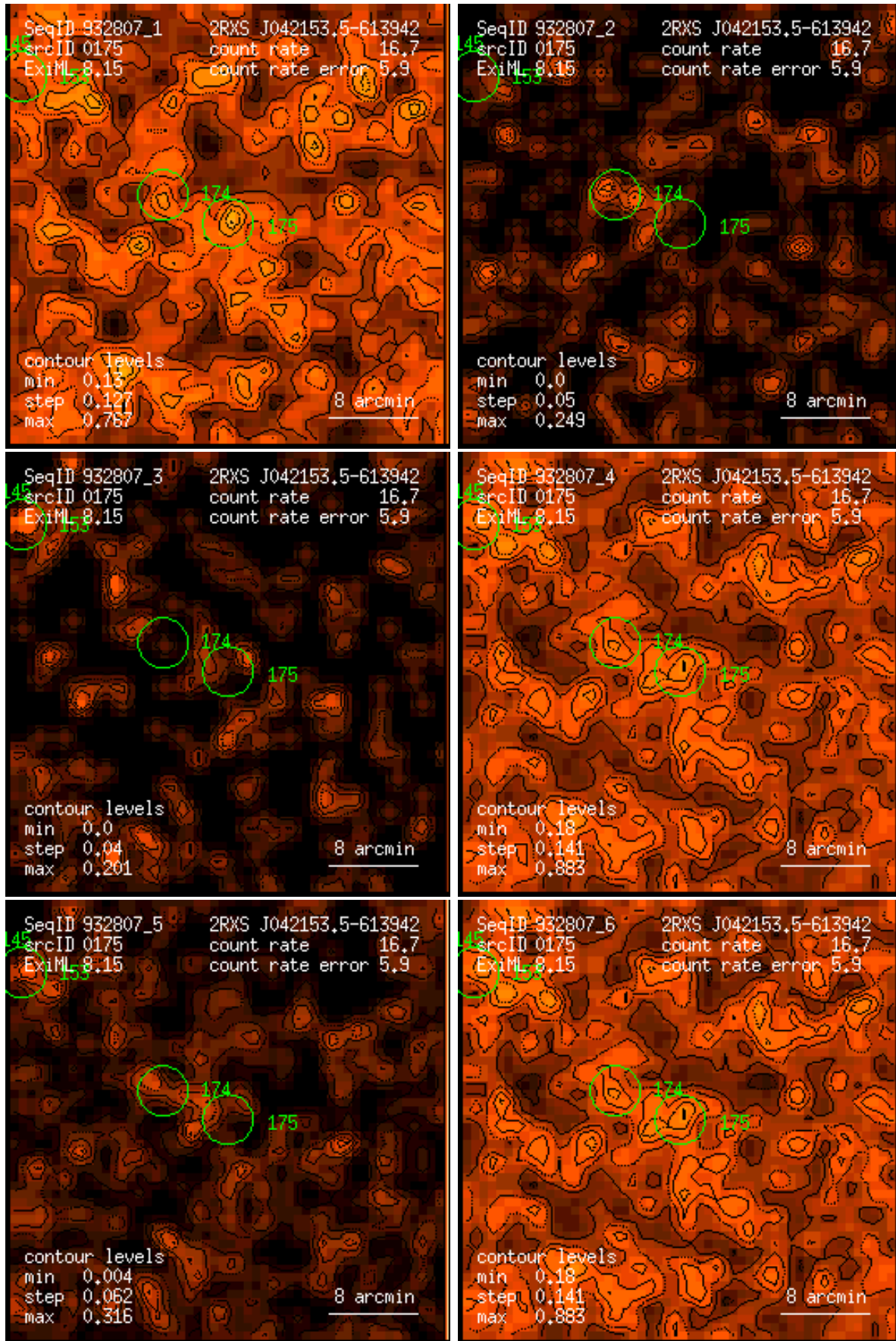
Figure 175: RASS 932807: detection 0175: band rate images, Gaussian filter: (1) PSPC channels 11 – 41, (2) 52 – 90, (3) 91 – 201, (4) 11 – 235, (5) 52 – 201, (6) 11 – 201. Broad band rates in counts/ks. Band rate contour levels in counts/ks/arcmin 2 .
