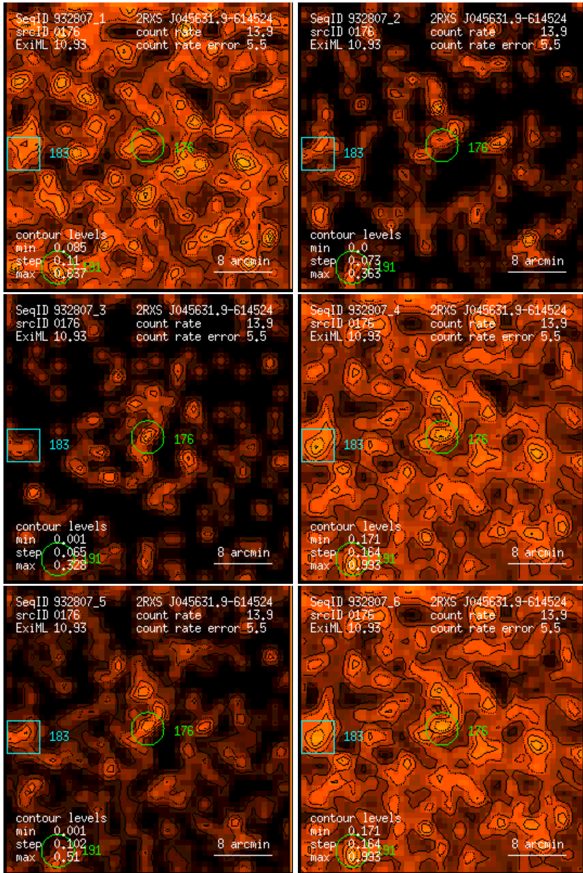
Figure 176: RASS 932807: detection 0176: band rate images, Gaussian filter: (1) PSPC channels 11 – 41, (2) 52 – 90, (3) 91 – 201, (4) 11 – 235, (5) 52 – 201, (6) 11 – 201. Broad band rates in counts/ks. Band rate contour levels in counts/ks/arcmin 2 .
