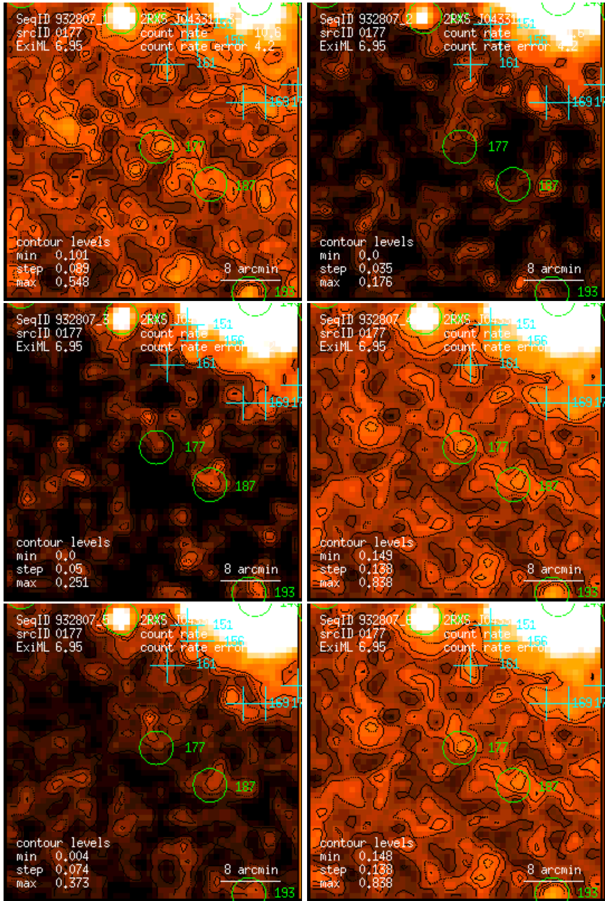
Figure 177: RASS 932807: detection 0177: band rate images, Gaussian filter: (1) PSPC channels 11 – 41, (2) 52 – 90, (3) 91 – 201, (4) 11 – 235, (5) 52 – 201, (6) 11 – 201. Broad band rates in counts/ks. Band rate contour levels in counts/ks/arcmin 2 .
