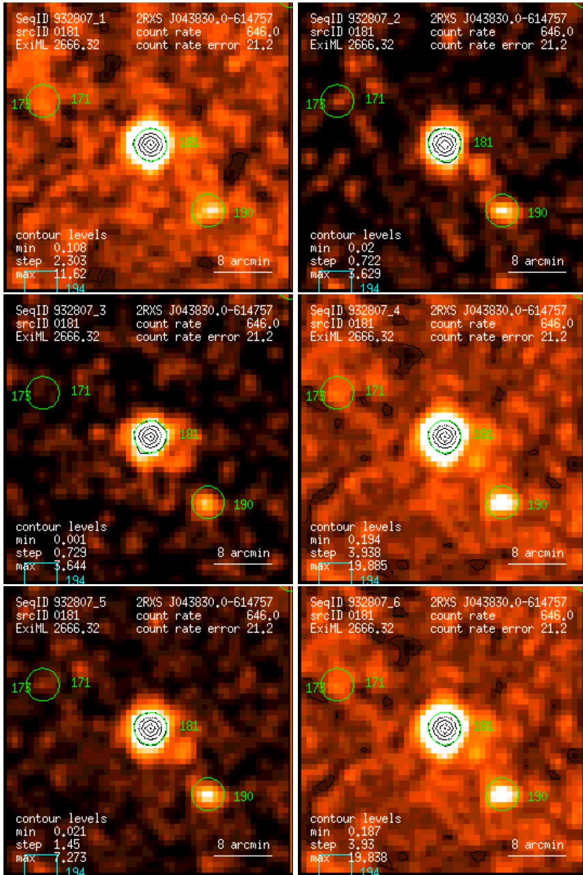
Figure 181: RASS 932807: detection 0181: band rate images, Gaussian filter: (1) PSPC channels 11 – 41, (2) 52 – 90, (3) 91 – 201, (4) 11 – 235, (5) 52 – 201, (6) 11 – 201. Broad band rates in counts/ks. Band rate contour levels in counts/ks/arcmin 2 .
