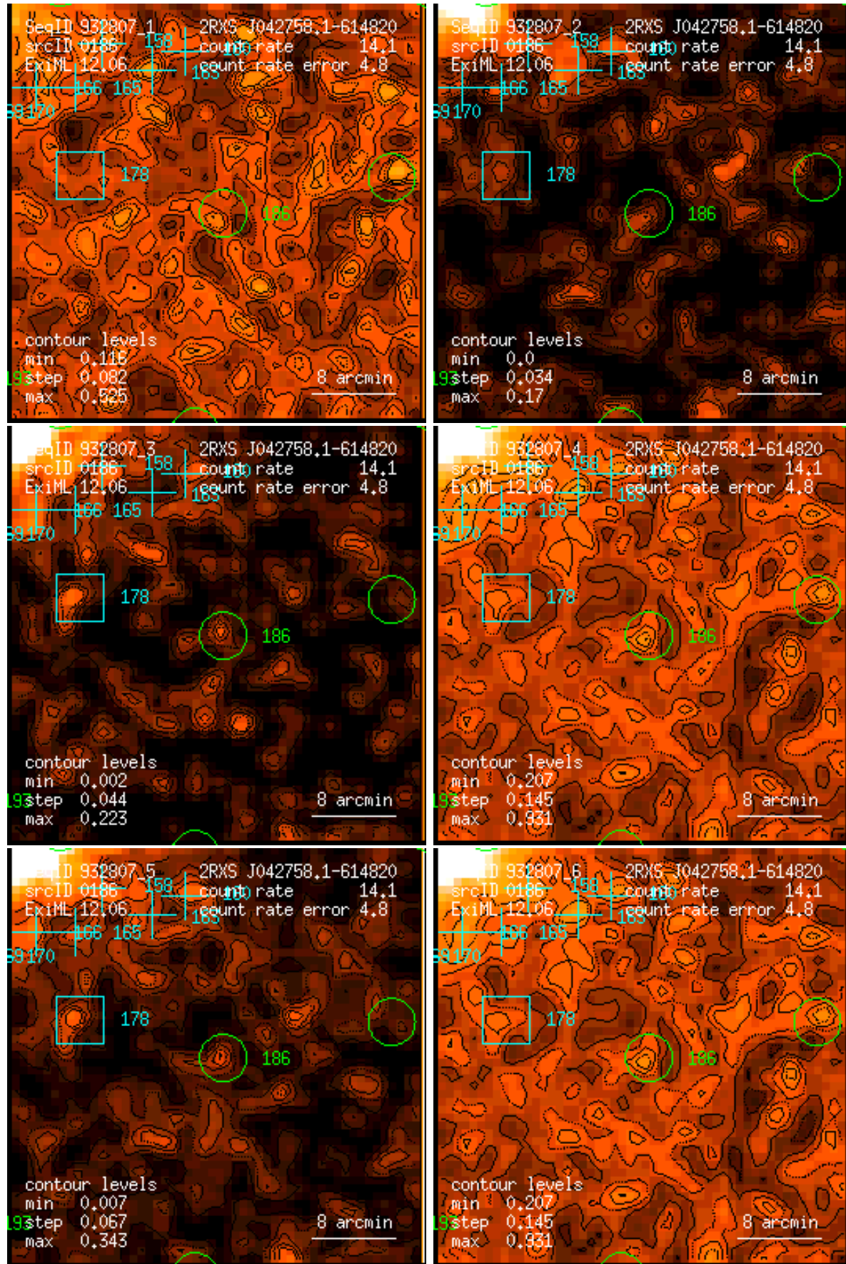
Figure 186: RASS 932807: detection 0186: band rate images, Gaussian filter: (1) PSPC channels 11 – 41, (2) 52 – 90, (3) 91 – 201, (4) 11 – 235, (5) 52 – 201, (6) 11 – 201. Broad band rates in counts/ks. Band rate contour levels in counts/ks/arcmin 2 .
