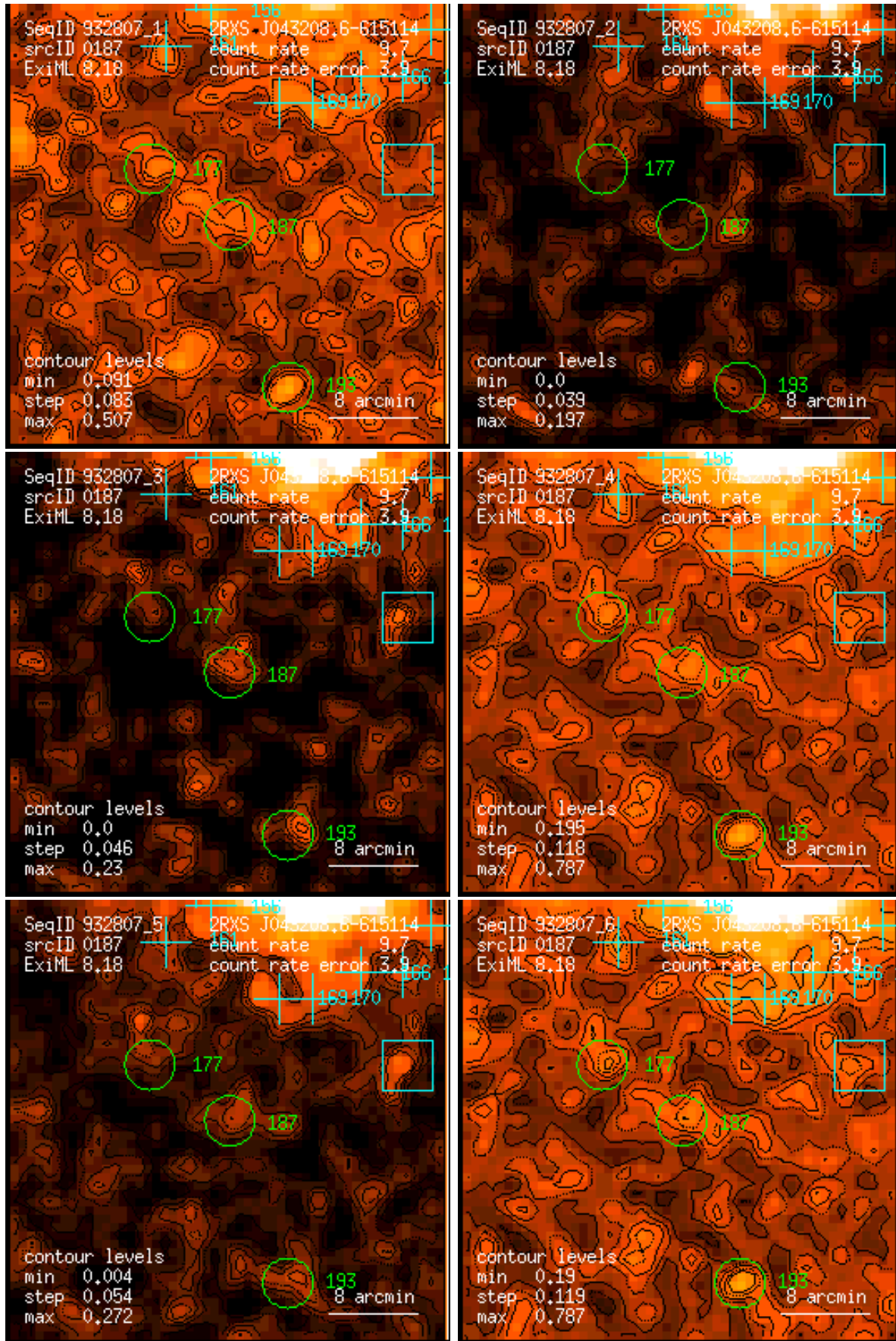
Figure 187: RASS 932807: detection 0187: band rate images, Gaussian filter: (1) PSPC channels 11 – 41, (2) 52 – 90, (3) 91 – 201, (4) 11 – 235, (5) 52 – 201, (6) 11 – 201. Broad band rates in counts/ks. Band rate contour levels in counts/ks/arcmin 2 .
