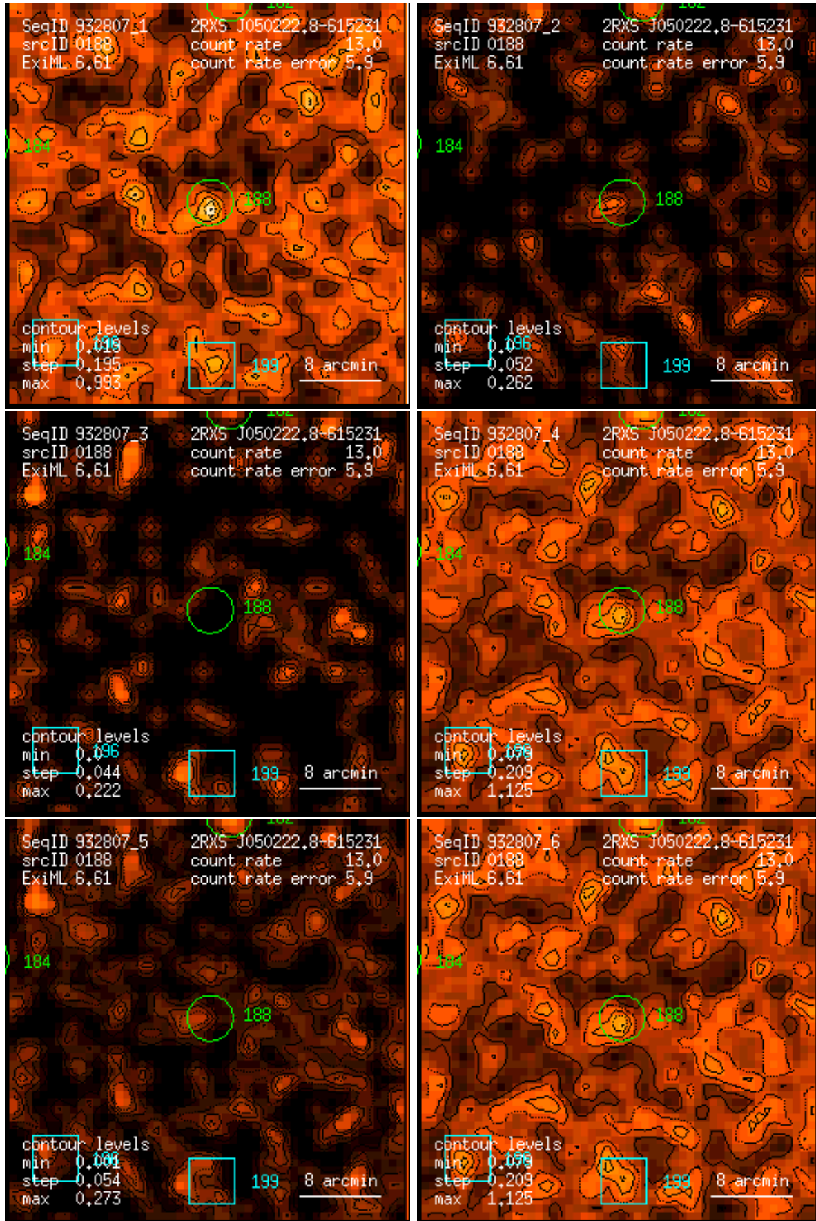
Figure 188: RASS 932807: detection 0188: band rate images, Gaussian filter: (1) PSPC channels 11 – 41, (2) 52 – 90, (3) 91 – 201, (4) 11 – 235, (5) 52 – 201, (6) 11 – 201. Broad band rates in counts/ks. Band rate contour levels in counts/ks/arcmin 2 .
