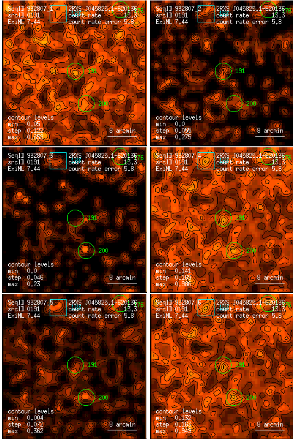
Figure 191: RASS 932807: detection 0191: band rate images, Gaussian filter: (1) PSPC channels 11 – 41, (2) 52 – 90, (3) 91 – 201, (4) 11 – 235, (5) 52 – 201, (6) 11 – 201. Broad band rates in counts/ks. Band rate contour levels in counts/ks/arcmin 2 .
