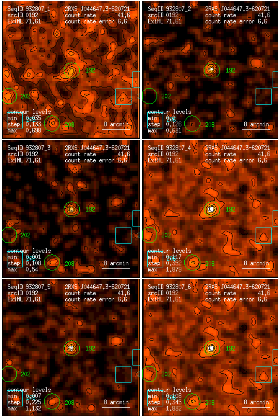
Figure 192: RASS 932807: detection 0192: band rate images, Gaussian filter: (1) PSPC channels 11 – 41, (2) 52 – 90, (3) 91 – 201, (4) 11 – 235, (5) 52 – 201, (6) 11 – 201. Broad band rates in counts/ks. Band rate contour levels in counts/ks/arcmin 2 .
