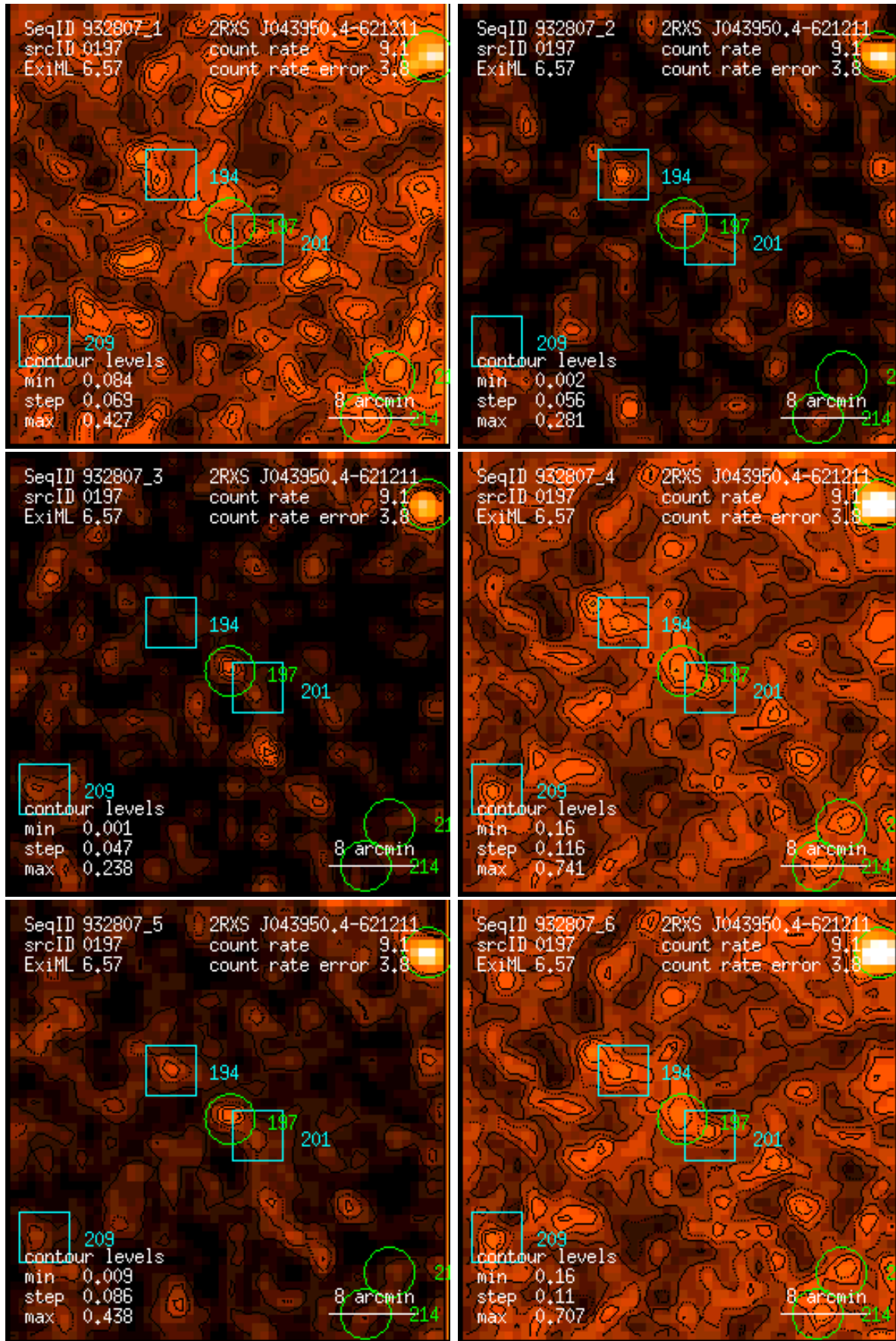
Figure 197: RASS 932807: detection 0197: band rate images, Gaussian filter: (1) PSPC channels 11 – 41, (2) 52 – 90, (3) 91 – 201, (4) 11 – 235, (5) 52 – 201, (6) 11 – 201. Broad band rates in counts/ks. Band rate contour levels in counts/ks/arcmin 2 .
