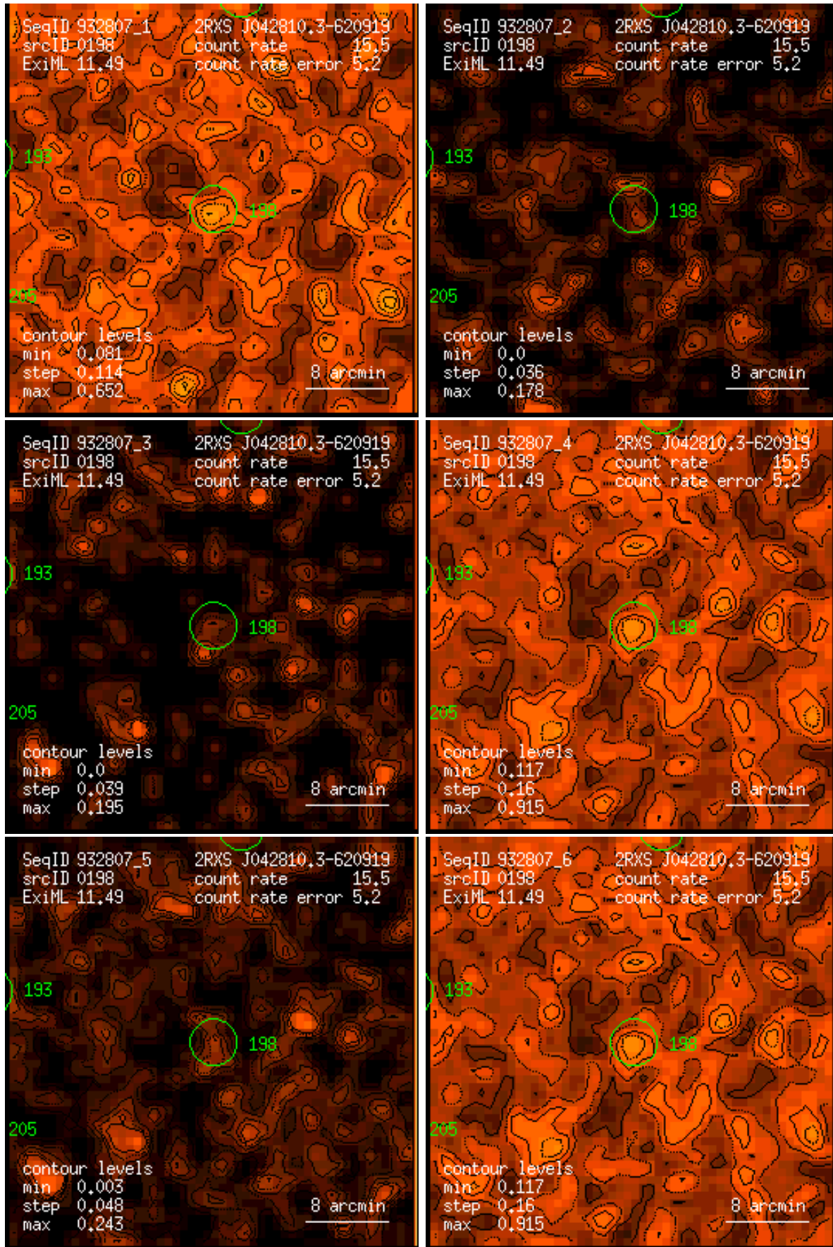
Figure 198: RASS 932807: detection 0198: band rate images, Gaussian filter: (1) PSPC channels 11 – 41, (2) 52 – 90, (3) 91 – 201, (4) 11 – 235, (5) 52 – 201, (6) 11 – 201. Broad band rates in counts/ks. Band rate contour levels in counts/ks/arcmin 2 .
