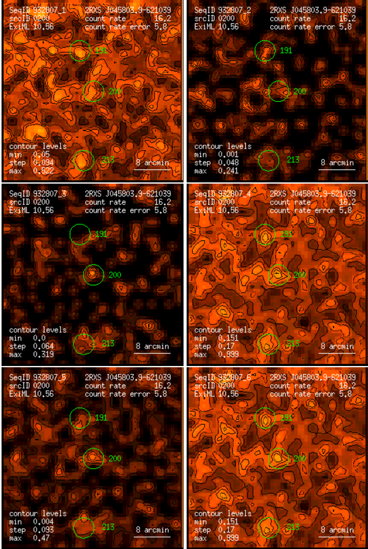
Figure 200: RASS 932807: detection 0200: band rate images, Gaussian filter: (1) PSPC channels 11 – 41, (2) 52 – 90, (3) 91 – 201, (4) 11 – 235, (5) 52 – 201, (6) 11 – 201. Broad band rates in counts/ks. Band rate contour levels in counts/ks/arcmin 2 .
