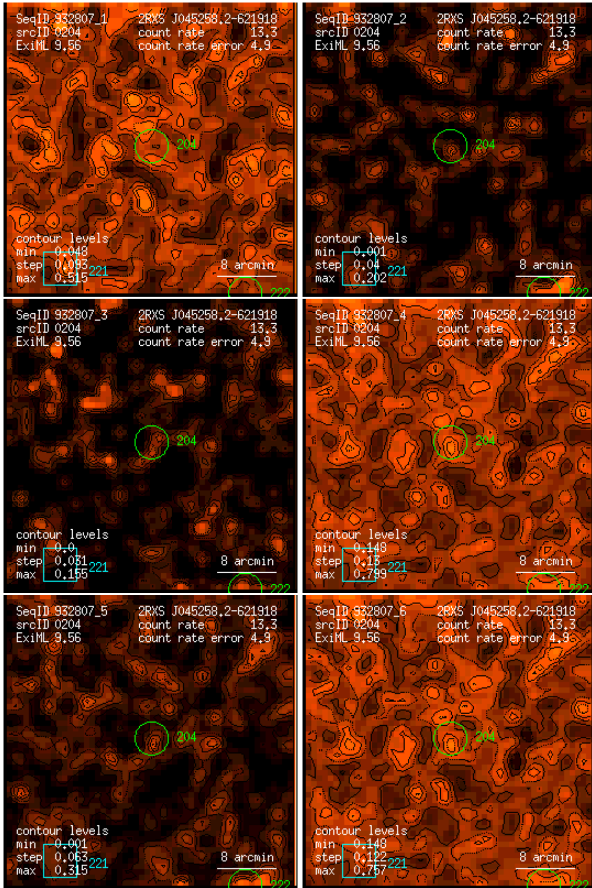
Figure 204: RASS 932807: detection 0204: band rate images, Gaussian filter: (1) PSPC channels 11 – 41, (2) 52 – 90, (3) 91 – 201, (4) 11 – 235, (5) 52 – 201, (6) 11 – 201. Broad band rates in counts/ks. Band rate contour levels in counts/ks/arcmin 2 .
