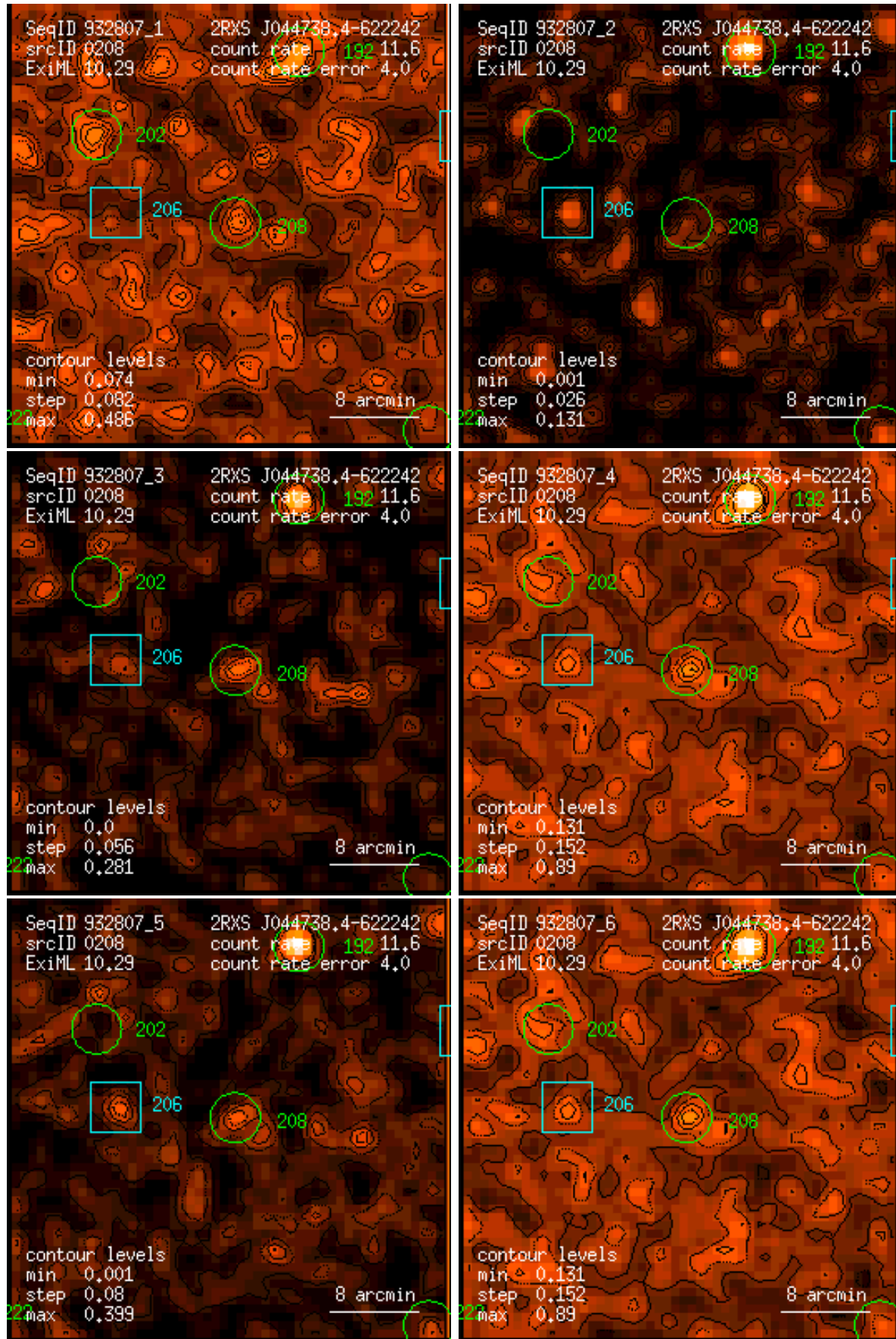
Figure 208: RASS 932807: detection 0208: band rate images, Gaussian filter: (1) PSPC channels 11 – 41, (2) 52 – 90, (3) 91 – 201, (4) 11 – 235, (5) 52 – 201, (6) 11 – 201. Broad band rates in counts/ks. Band rate contour levels in counts/ks/arcmin 2 .
