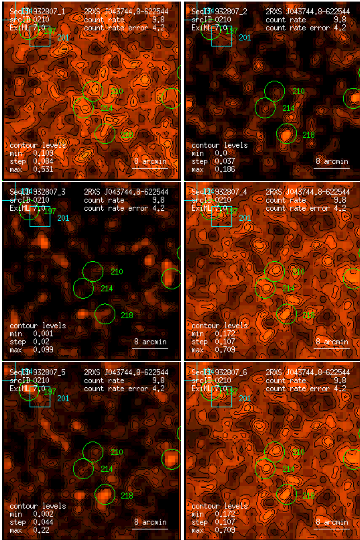
Figure 210: RASS 932807: detection 0210: band rate images, Gaussian filter: (1) PSPC channels 11 – 41, (2) 52 – 90, (3) 91 – 201, (4) 11 – 235, (5) 52 – 201, (6) 11 – 201. Broad band rates in counts/ks. Band rate contour levels in counts/ks/arcmin 2 .
