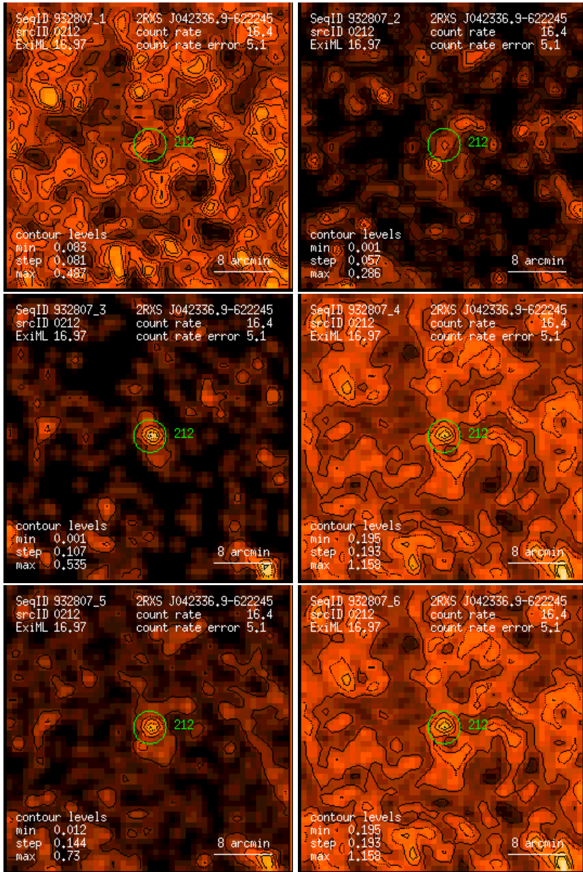
Figure 212: RASS 932807: detection 0212: band rate images, Gaussian filter: (1) PSPC channels 11 – 41, (2) 52 – 90, (3) 91 – 201, (4) 11 – 235, (5) 52 – 201, (6) 11 – 201. Broad band rates in counts/ks. Band rate contour levels in counts/ks/arcmin 2 .
