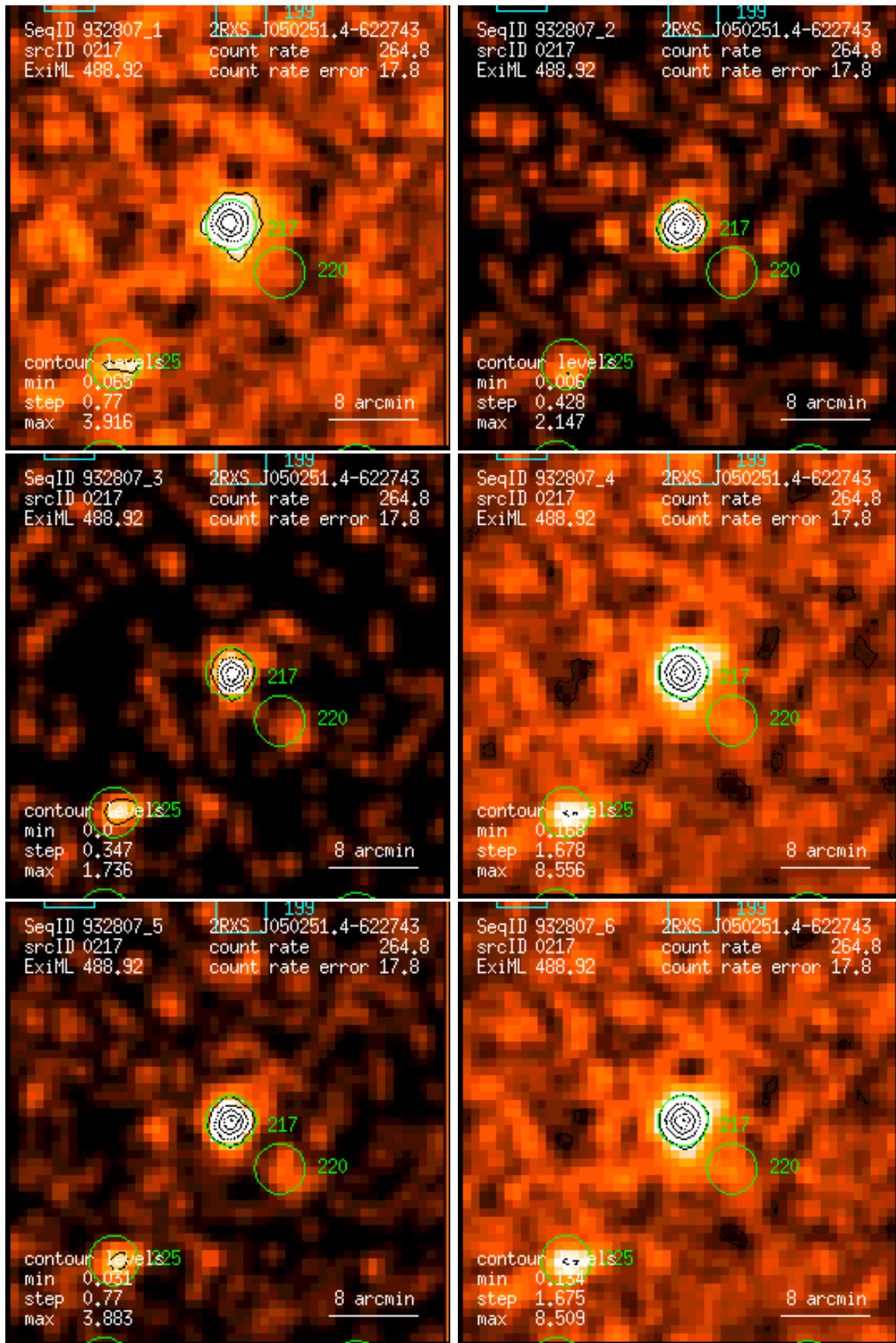
Figure 217: RASS 932807: detection 0217: band rate images, Gaussian filter: (1) PSPC channels 11 – 41, (2) 52 – 90, (3) 91 – 201, (4) 11 – 235, (5) 52 – 201, (6) 11 – 201. Broad band rates in counts/ks. Band rate contour levels in counts/ks/arcmin 2 .
