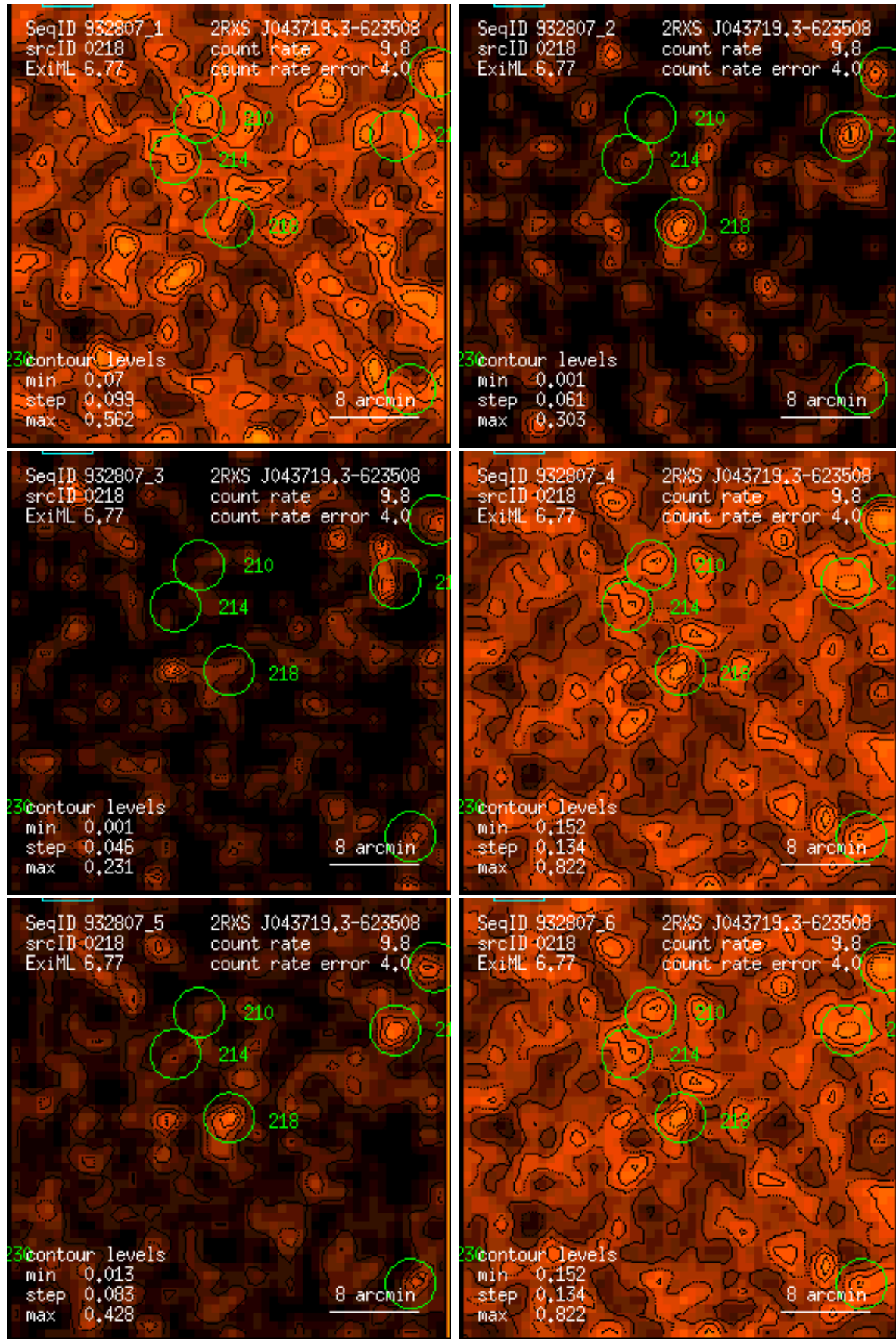
Figure 218: RASS 932807: detection 0218: band rate images, Gaussian filter: (1) PSPC channels 11 – 41, (2) 52 – 90, (3) 91 – 201, (4) 11 – 235, (5) 52 – 201, (6) 11 – 201. Broad band rates in counts/ks. Band rate contour levels in counts/ks/arcmin 2 .
