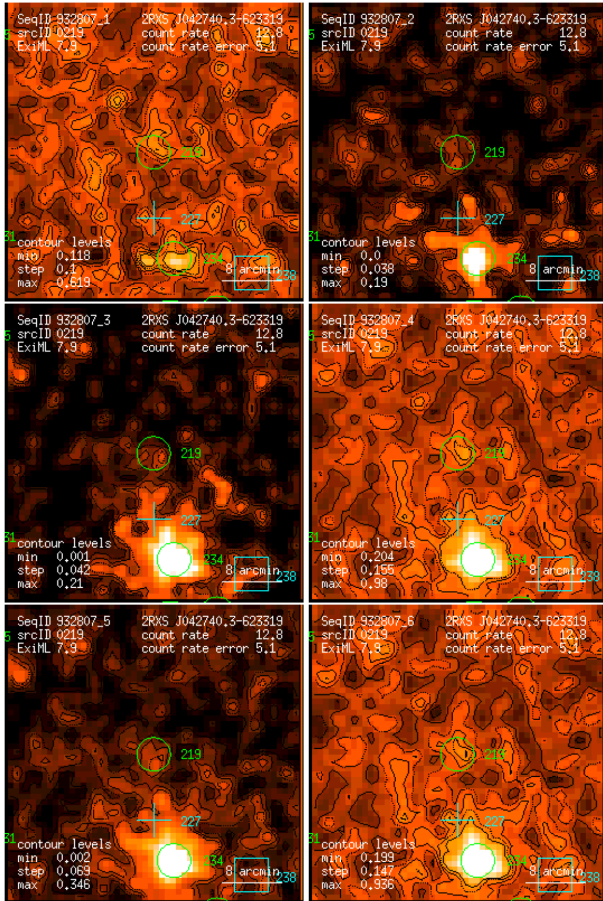
Figure 219: RASS 932807: detection 0219: band rate images, Gaussian filter: (1) PSPC channels 11 – 41, (2) 52 – 90, (3) 91 – 201, (4) 11 – 235, (5) 52 – 201, (6) 11 – 201. Broad band rates in counts/ks. Band rate contour levels in counts/ks/arcmin 2 .
