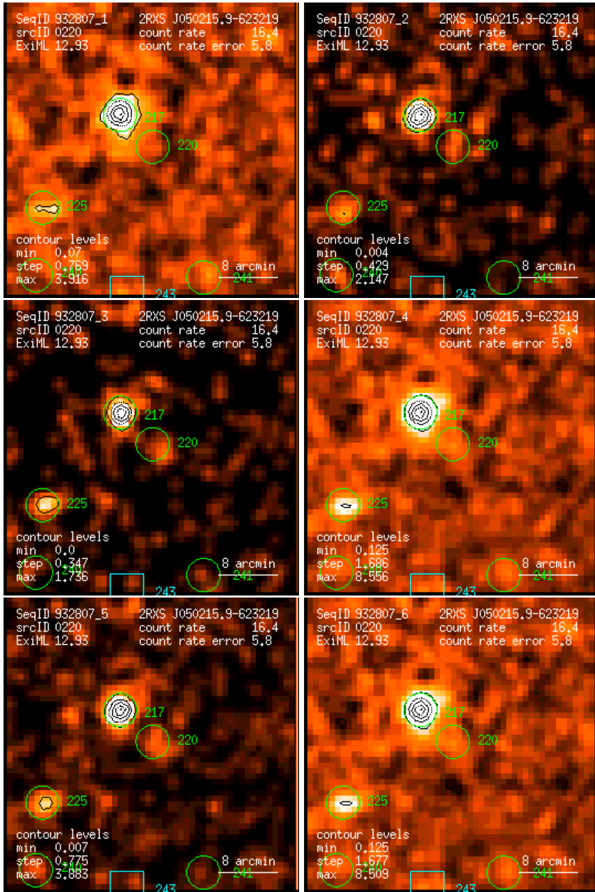
Figure 220: RASS 932807: detection 0220: band rate images, Gaussian filter: (1) PSPC channels 11 – 41, (2) 52 – 90, (3) 91 – 201, (4) 11 – 235, (5) 52 – 201, (6) 11 – 201. Broad band rates in counts/ks. Band rate contour levels in counts/ks/arcmin 2 .
