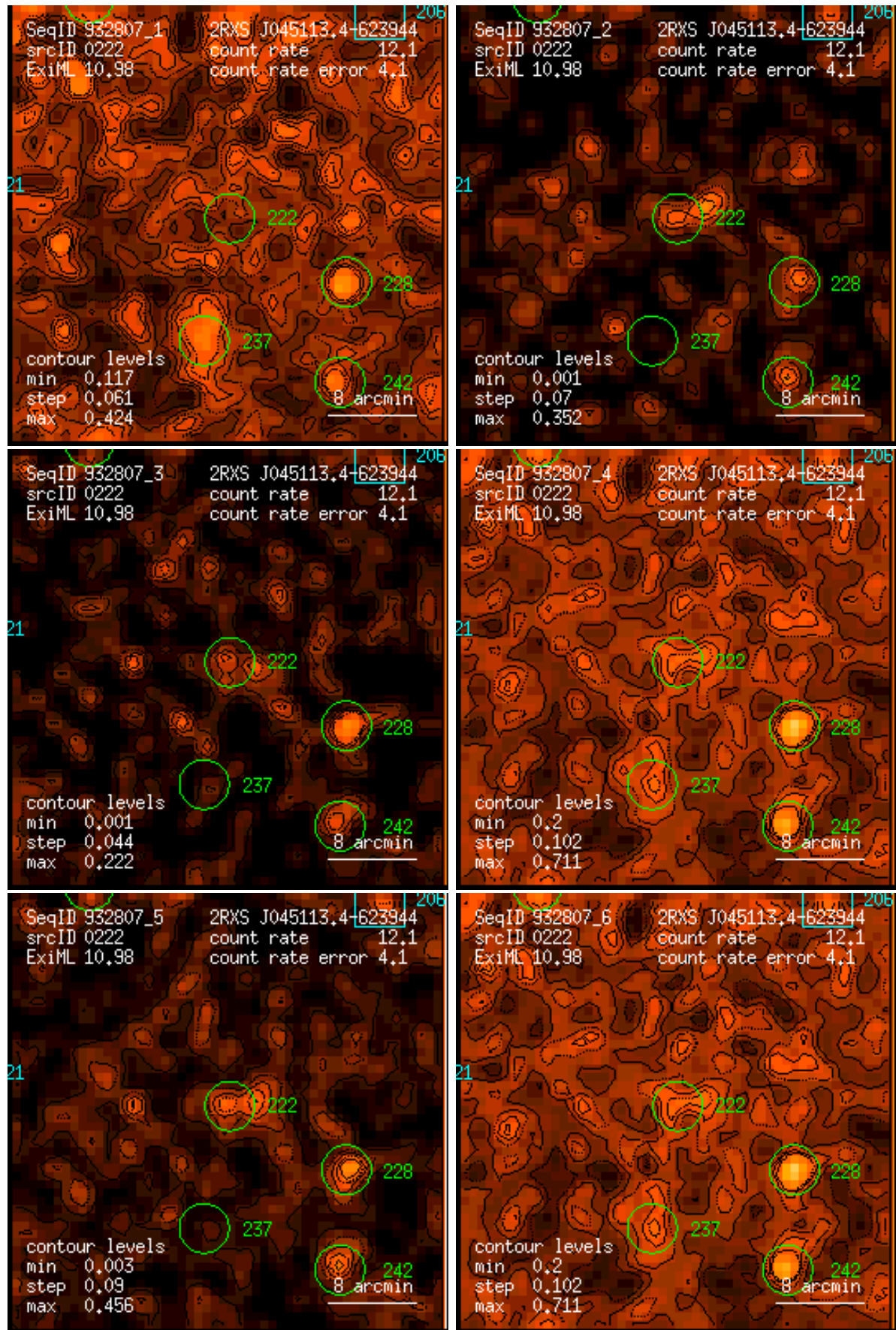
Figure 222: RASS 932807: detection 0222: band rate images, Gaussian filter: (1) PSPC channels 11 – 41, (2) 52 – 90, (3) 91 – 201, (4) 11 – 235, (5) 52 – 201, (6) 11 – 201. Broad band rates in counts/ks. Band rate contour levels in counts/ks/arcmin 2 .
