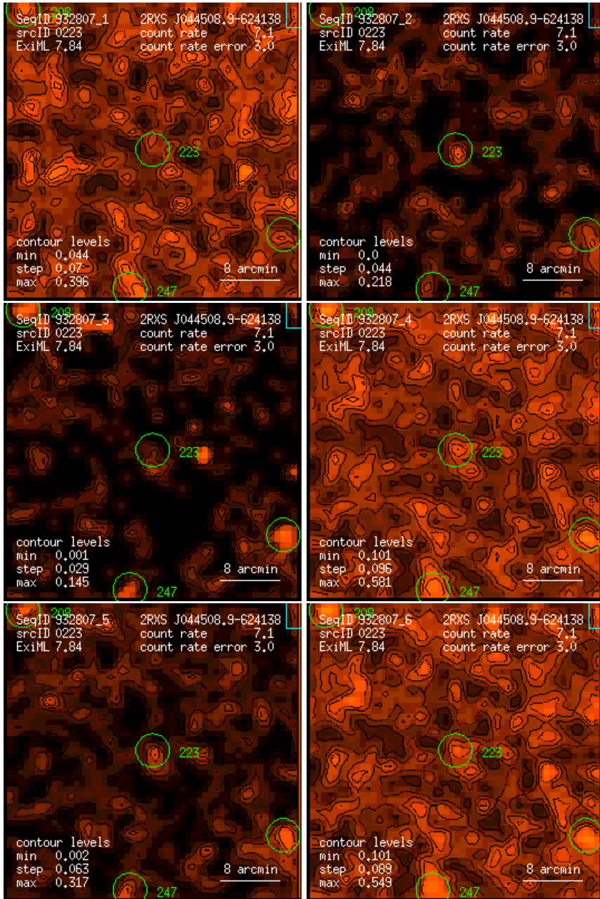
Figure 223: RASS 932807: detection 0223: band rate images, Gaussian filter: (1) PSPC channels 11 – 41, (2) 52 – 90, (3) 91 – 201, (4) 11 – 235, (5) 52 – 201, (6) 11 – 201. Broad band rates in counts/ks. Band rate contour levels in counts/ks/arcmin 2 .
