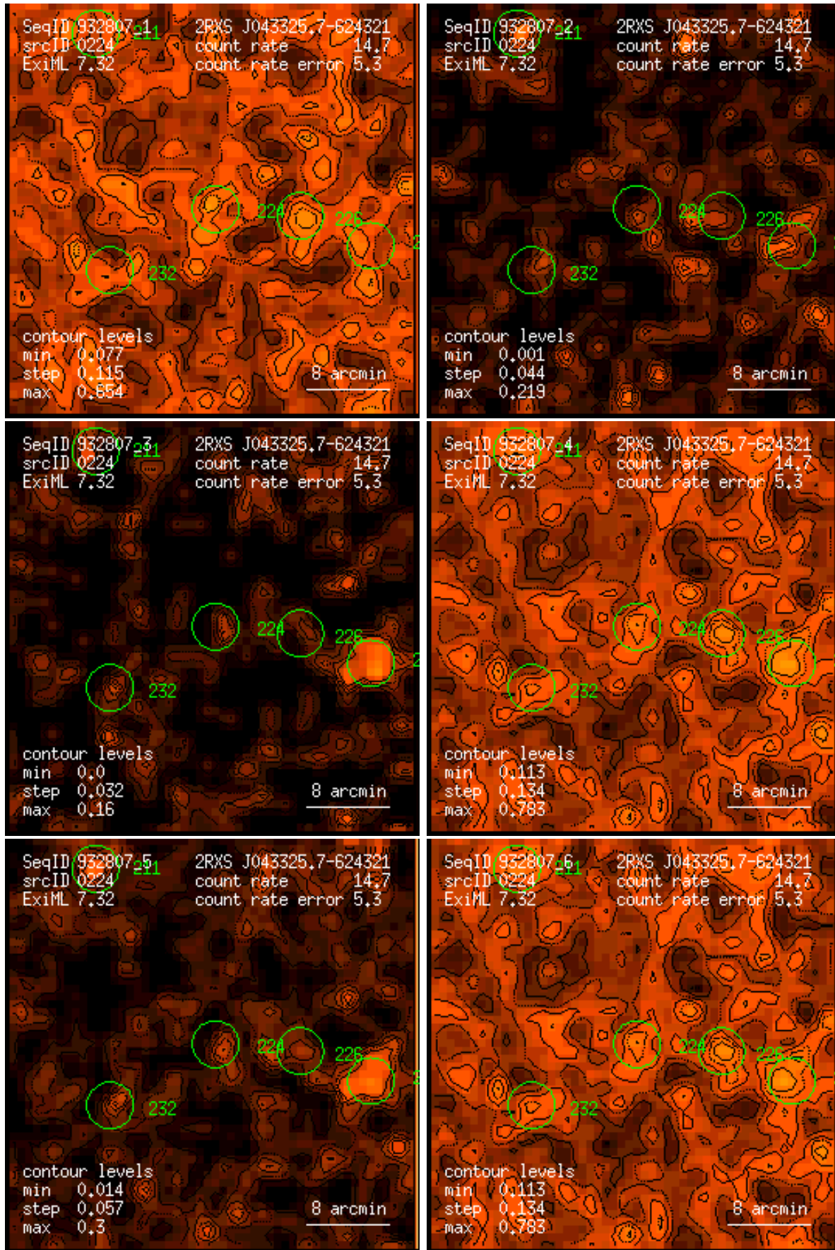
Figure 224: RASS 932807: detection 0224: band rate images, Gaussian filter: (1) PSPC channels 11 – 41, (2) 52 – 90, (3) 91 – 201, (4) 11 – 235, (5) 52 – 201, (6) 11 – 201. Broad band rates in counts/ks. Band rate contour levels in counts/ks/arcmin 2 .
