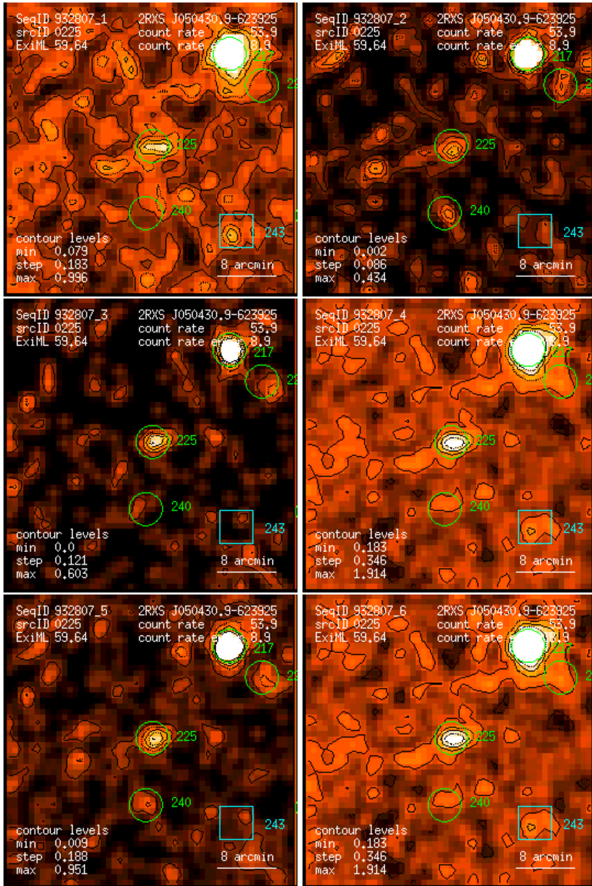
Figure 225: RASS 932807: detection 0225: band rate images, Gaussian filter: (1) PSPC channels 11 – 41, (2) 52 – 90, (3) 91 – 201, (4) 11 – 235, (5) 52 – 201, (6) 11 – 201. Broad band rates in counts/ks. Band rate contour levels in counts/ks/arcmin 2 .
