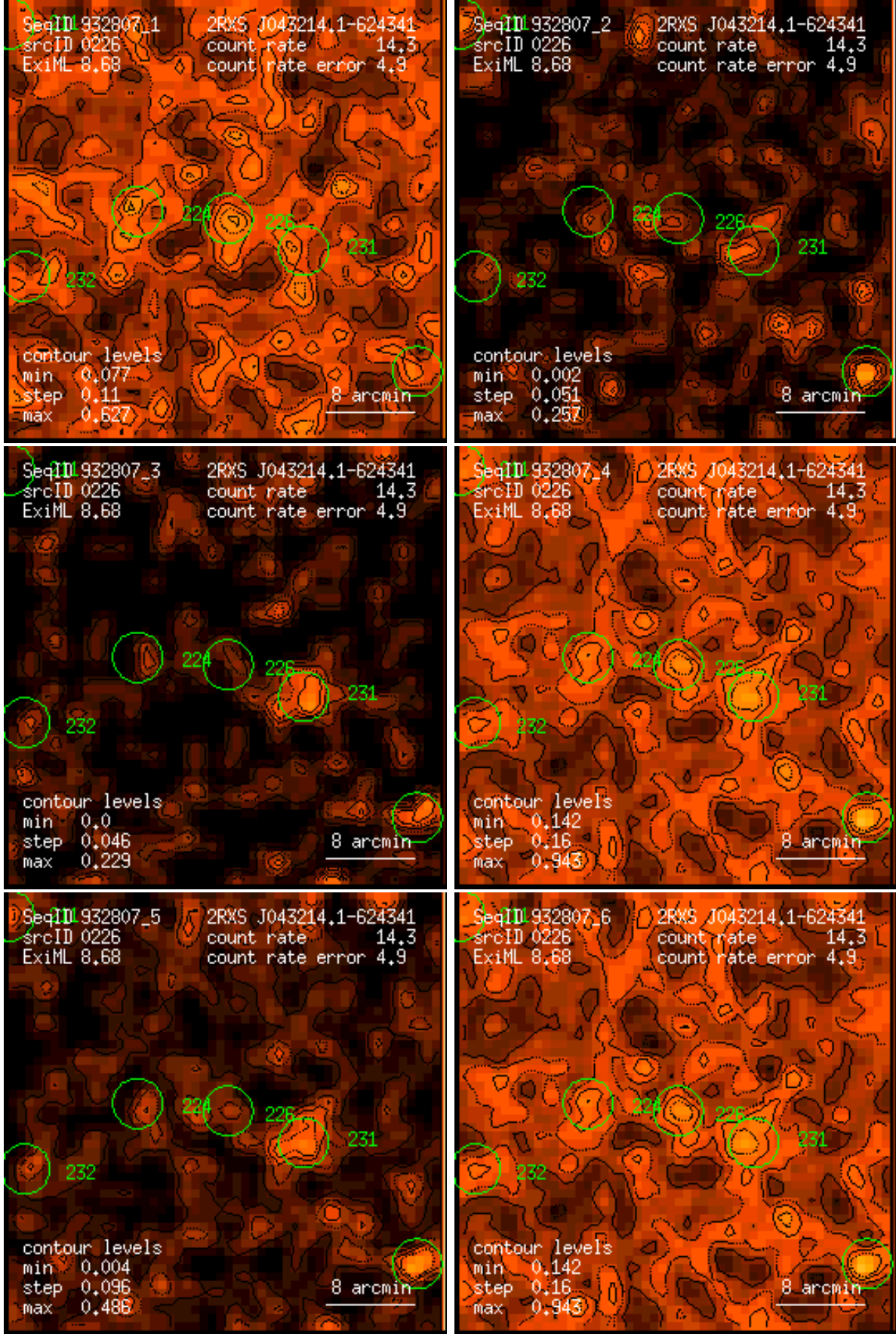
Figure 226: RASS 932807: detection 0226: band rate images, Gaussian filter: (1) PSPC channels 11 – 41, (2) 52 – 90, (3) 91 – 201, (4) 11 – 235, (5) 52 – 201, (6) 11 – 201. Broad band rates in counts/ks. Band rate contour levels in counts/ks/arcmin 2 .
