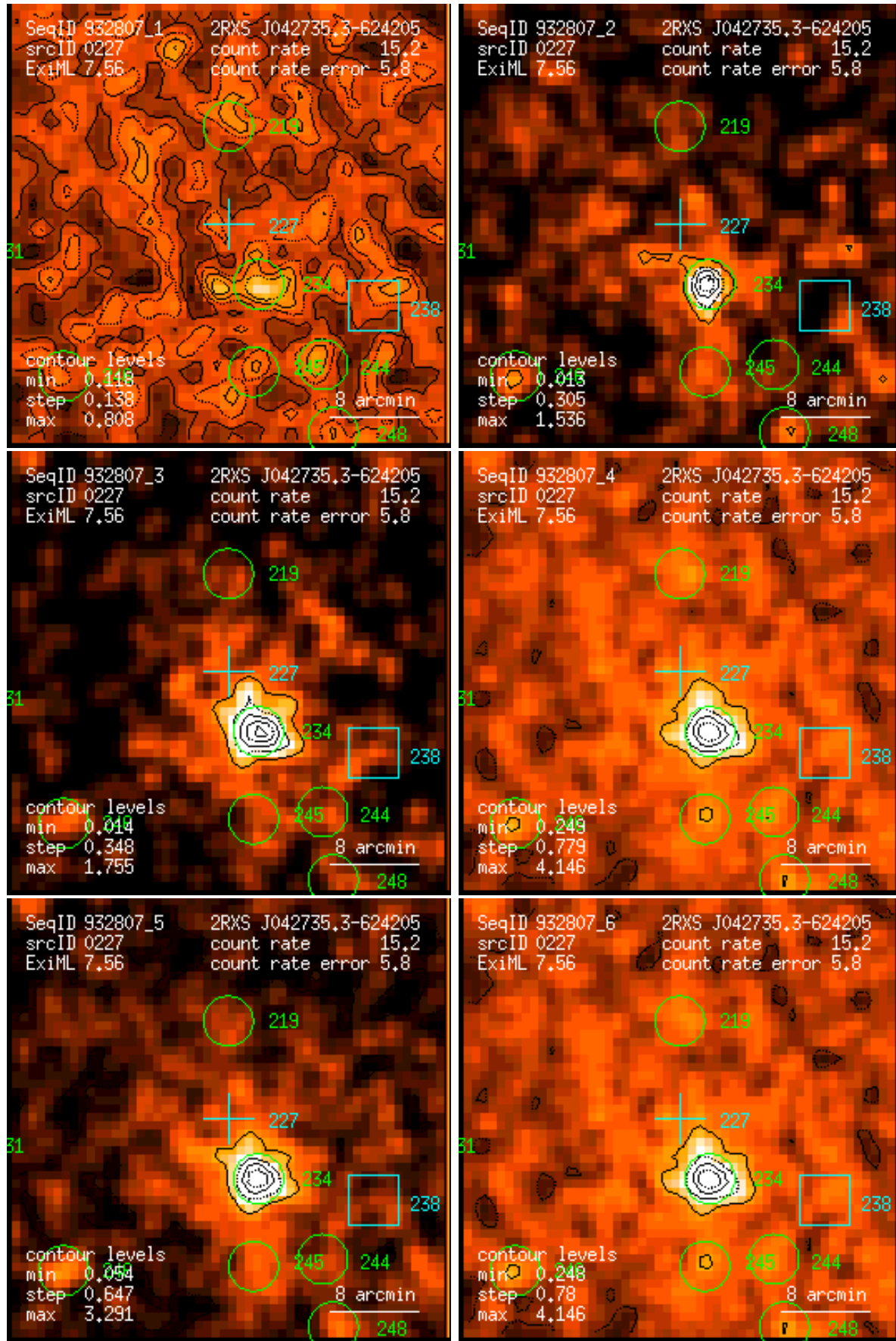
Figure 227: RASS 932807: detection 0227: band rate images, Gaussian filter: (1) PSPC channels 11 – 41, (2) 52 – 90, (3) 91 – 201, (4) 11 – 235, (5) 52 – 201, (6) 11 – 201. Broad band rates in counts/ks. Band rate contour levels in counts/ks/arcmin 2 .
